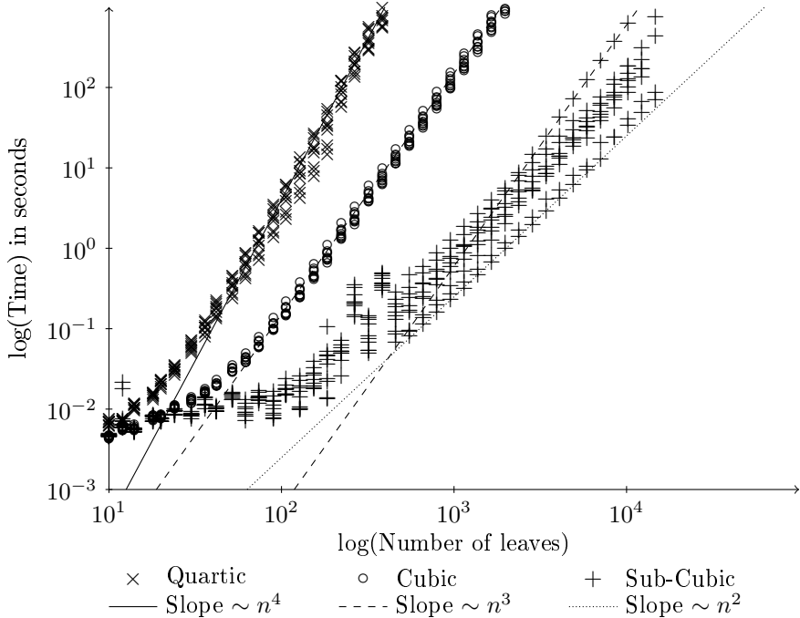
Number of leaves versus execution time
