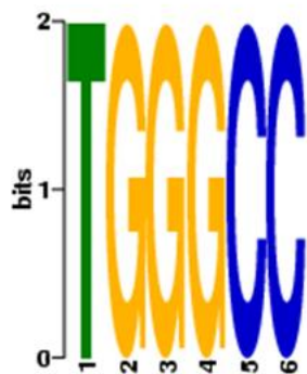
(c) Potential NAC TF Binding Motif3
