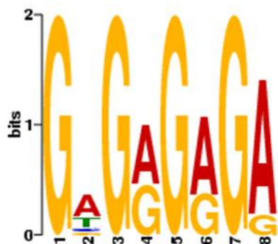
(b) Potential NAC TF Binding Motif2
