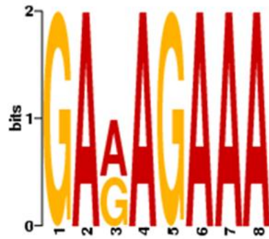
(f) Potential YABBY family TF Binding Motif3
