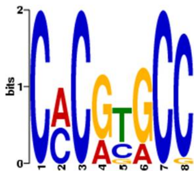
(c) Potential NAC TF Binding Motif3
