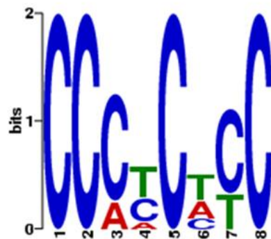
(e) Potential YABBY TF Binding Motif2
