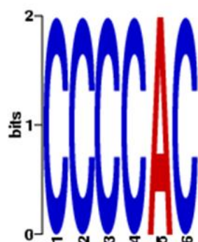
(f) Potential YABBY family TF Binding Motif3
