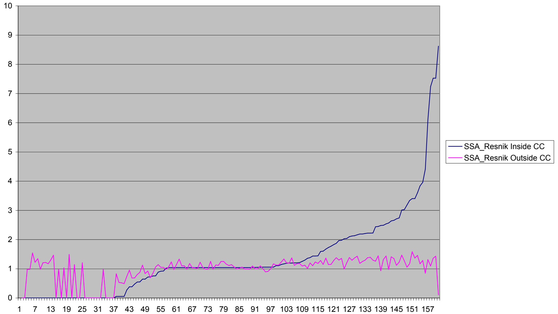
SSA_Resnik Average Similarity Values for Cellular Component Terms Only
