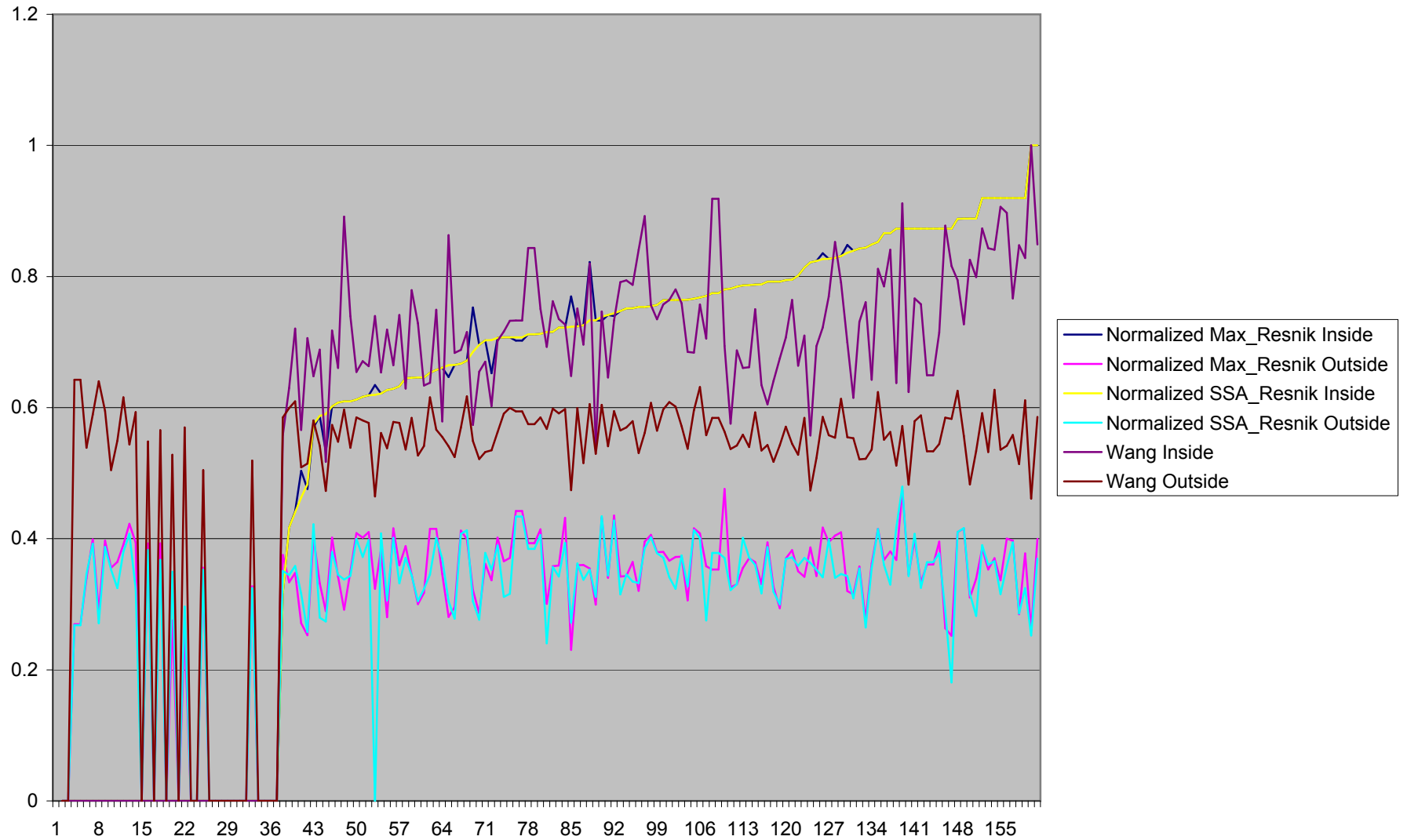
Average Similarity Values Inside and Outside Pathways - All Terms (CC, BP and MF)
