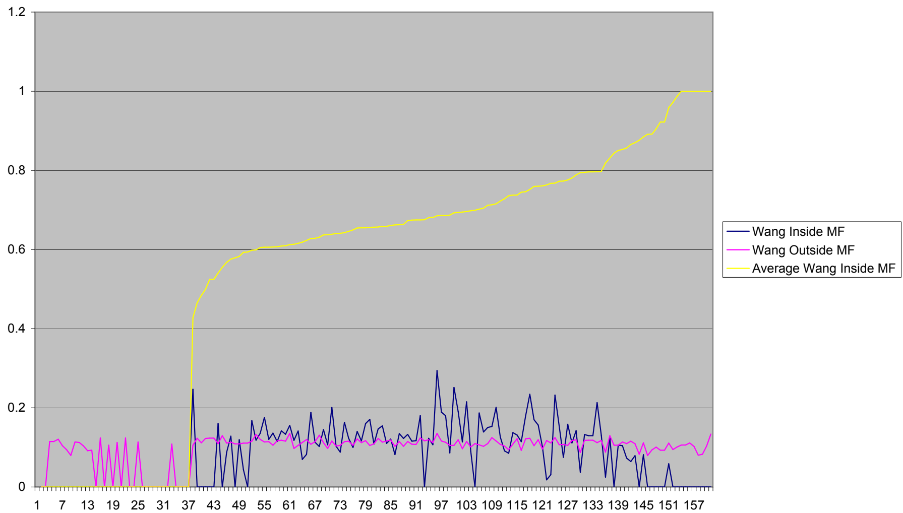
Wang Standard Deviation of Similarity Values for Molecular Function Terms Only
