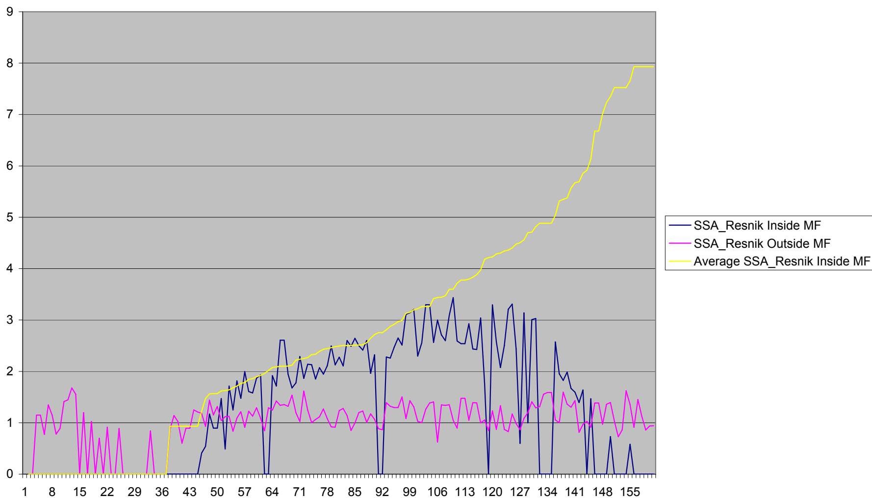
SSA_Resnik Standard Deviation of Similarity Values for Molecular Function Terms Only
