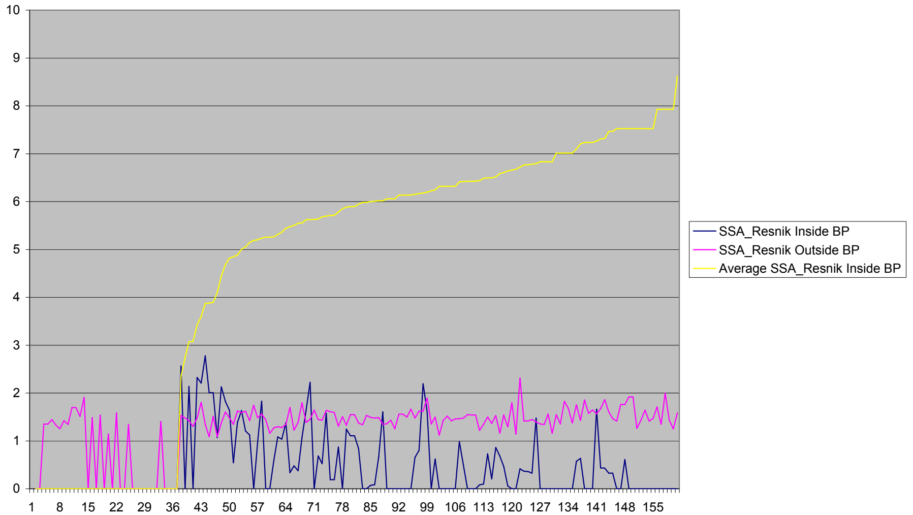
SSA_Resnik Standard Deviation of Similarity Values for Biological Process Terms Only
