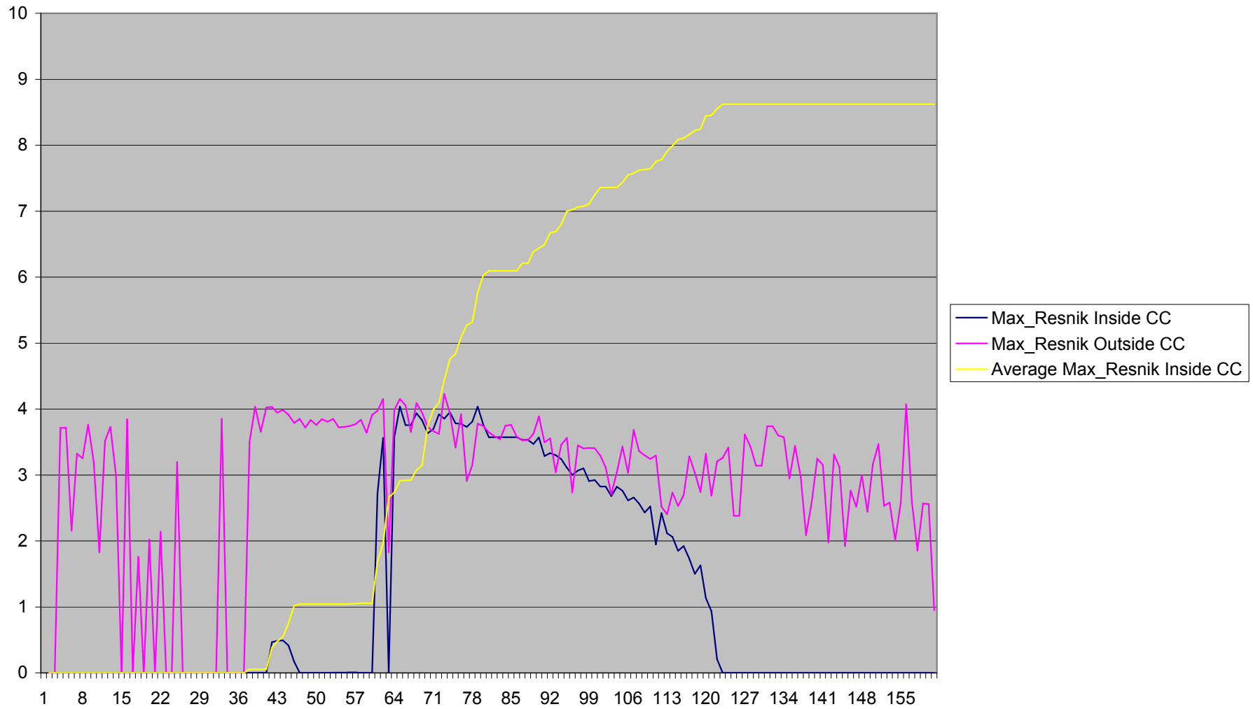
Max_Resnik Standard Deviation of Similarity Values for Cellular Component Terms Only
