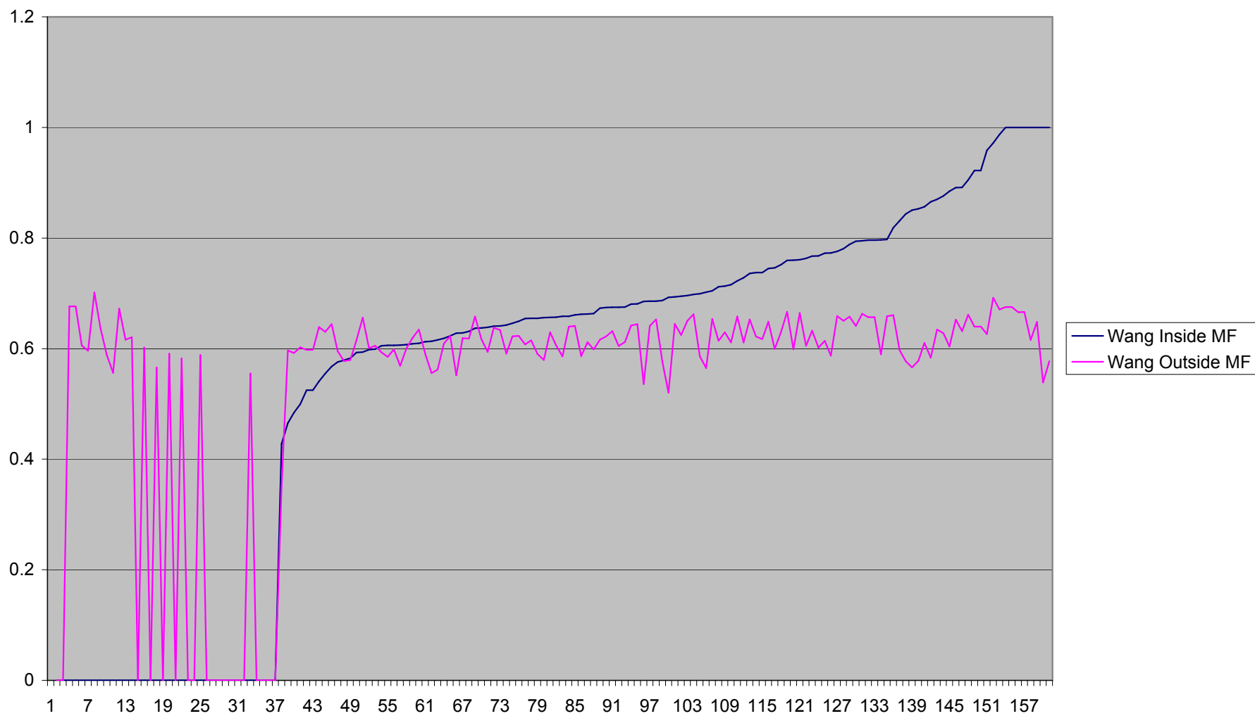
Wang Average Similarity Values for Molecular Function Terms Only
