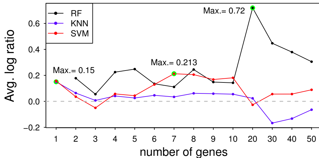
Avg. log ratio across considered data sets
