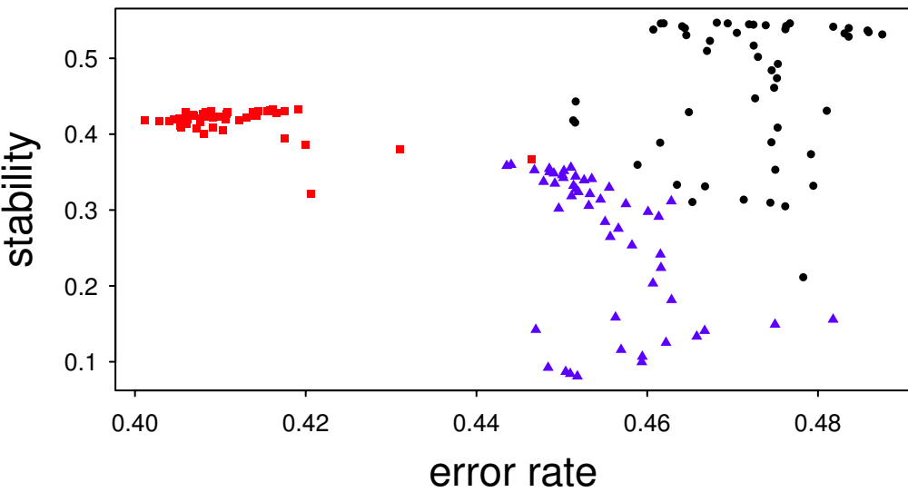
RF
