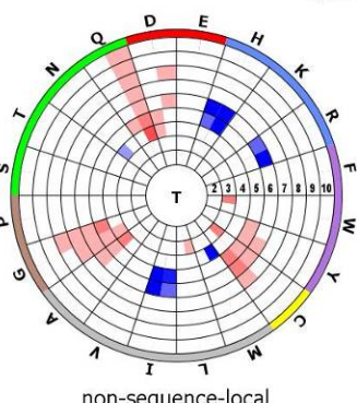
non-sequence-local
