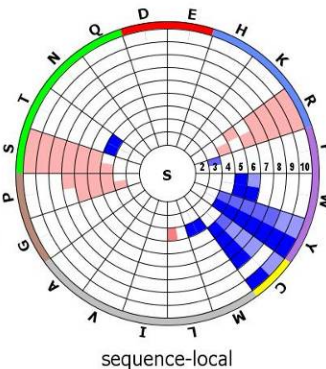
sequence-local
