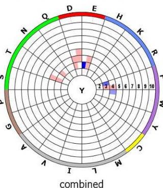
combined
