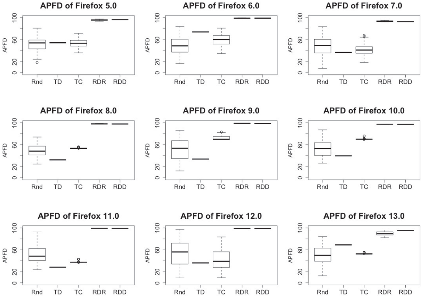
Fig. 4. Distribution of the APFDs of the five TCPs on nine rapid releases, over 100 runs, as boxplots.
