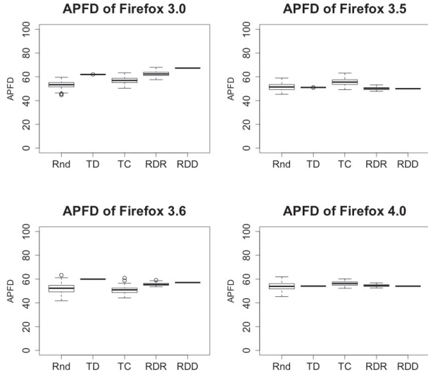
Fig. 3. Distribution of the APFDs of the five TCPS on four traditional releases, over 100 runs, as boxplots.
