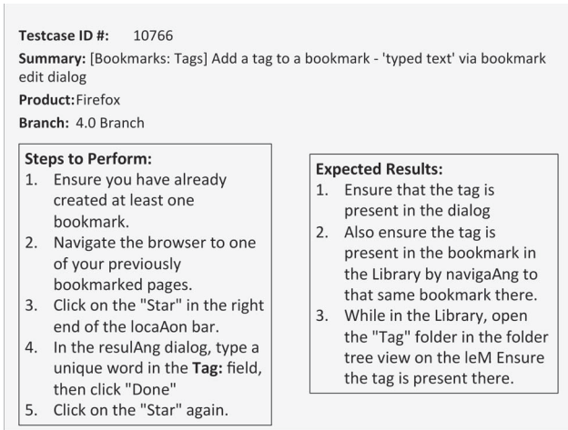
Fig. 1. A typical manual system-level test case in Mozilla Firefox project.
