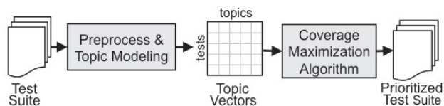
Fig. 2. Overview of our proposed topic-based TCP technique.
