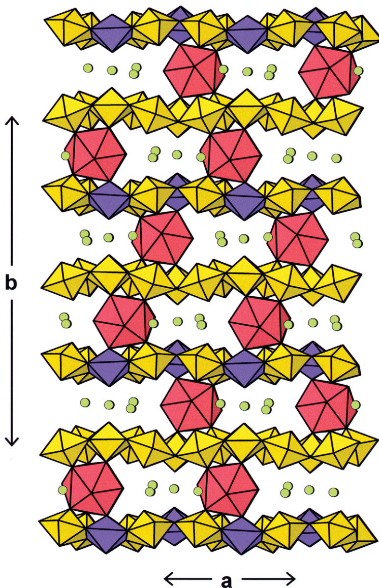
FIG. 2. The crystal structure of billietite projected down the c axis. Legend as in Figure 1; the Ba polyhedra are shown in red, and the interstitial ( H_2O ) groups are shown as green circles.
