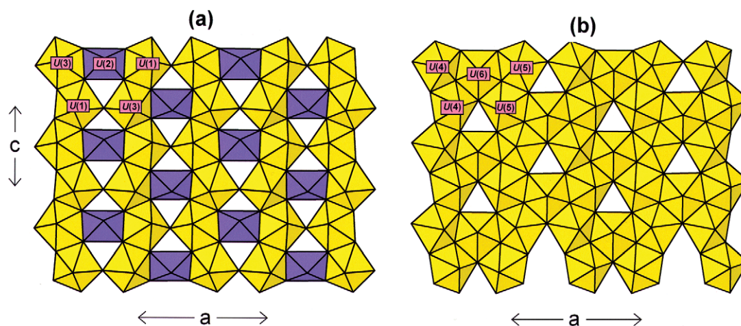
FIG. 1. The structural sheets of uranyl polyhedra in billietite projected along the b axis; (a) sheet of U (1), U (2) and U (3) polyhedra; (b) sheet of U (4), U (5), and U (6) polyhedra; U (2): mauve; other U polyhedra: yellow.
