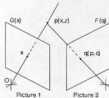
Figure 3: Stereo vision
