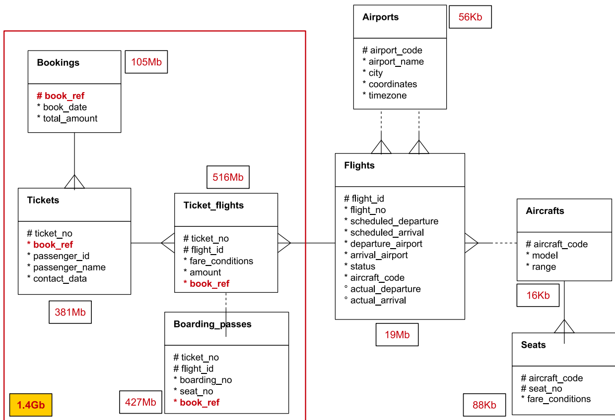
Figure 16.4. Source Schema Modification
