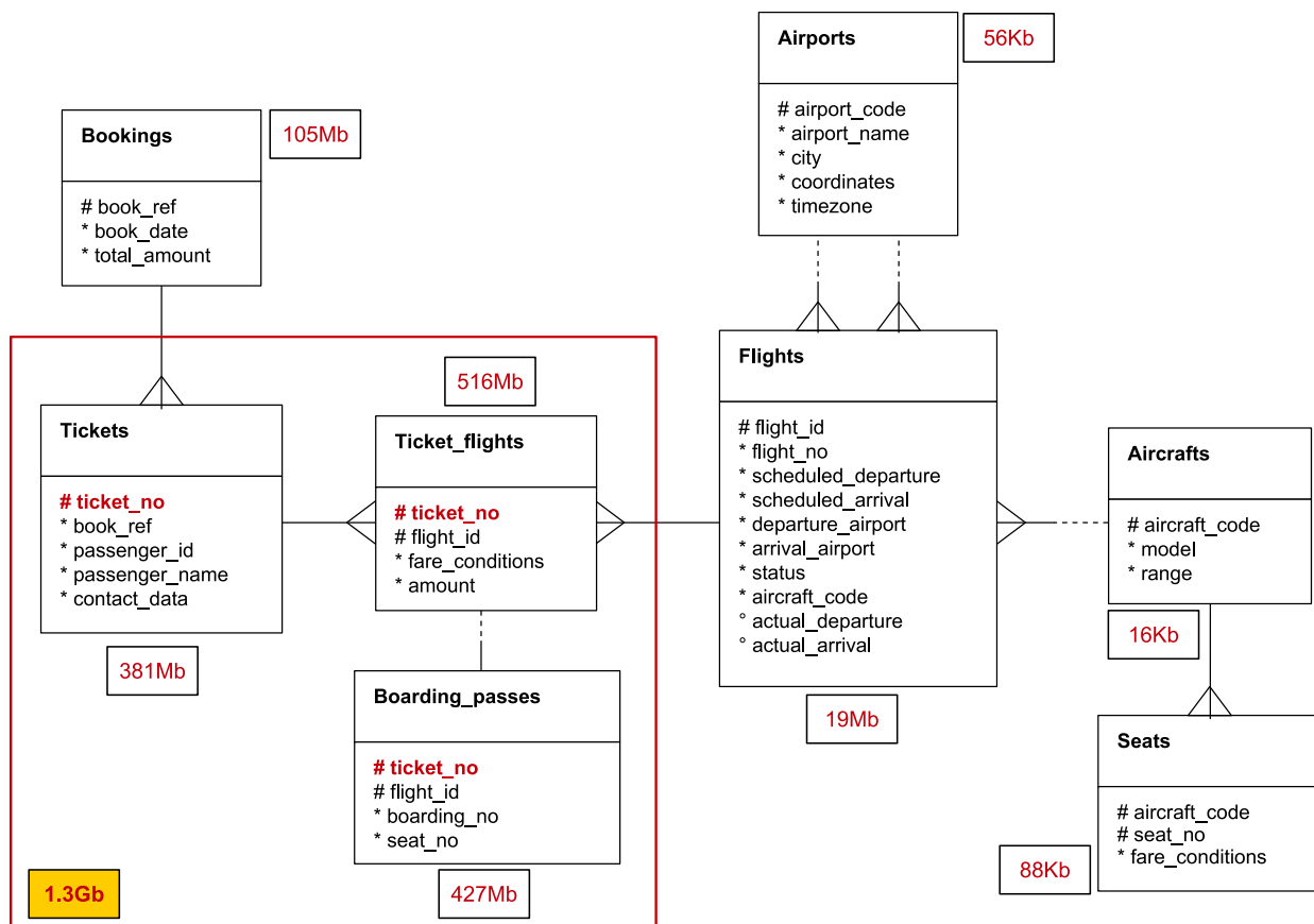
Figure 16.3. Naive Approach Schema
