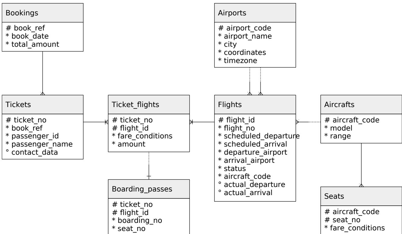
Figure 16.2. Database Source Schema
