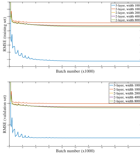
Figure 1. The experiment results, depicting the network’s root mean square error over the training set (top) and validation set (bottom), as a function of the number of batches processed. Best viewed in color.
