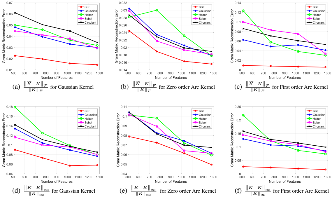
Figure 3. Relative Mean and Max Reconstruction Error for Gaussian, Zero-order and First-order Arc-cosine Kernel on uspst
