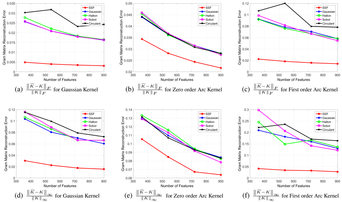
Figure 2. Relative Mean and Max Reconstruction Error for Gaussian, Zero-order and First-order Arc-cosine Kernel on dna
