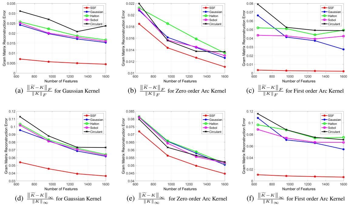
Figure 1. Relative Mean and Max Reconstruction Error for Gaussian, Zero-order and First-order Arc-cosine Kernel on CIFAR10
