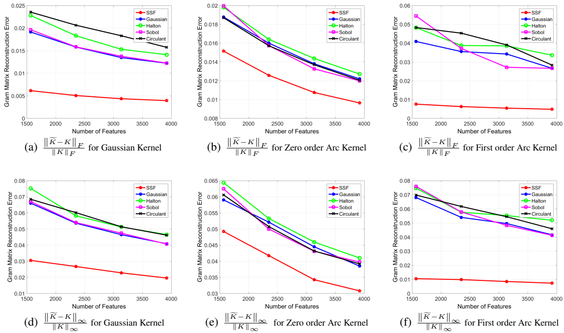
Figure 4. Relative Mean and Max Reconstruction Error for Gaussian, zero and first order arc-cosine Kernel on MNIST
