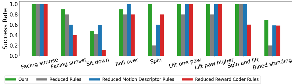
Figure 5: Ablation study for different amount of rules in the designed prompts.
