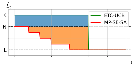
Figure 2. The update of candidate set's expected size \tilde{L}_t
