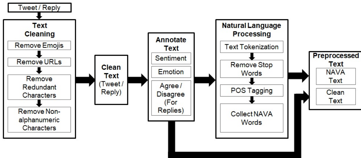
Figure 4.2: Preprocessing Workflow.
