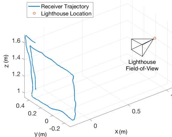
Fig. 8. Illustration of lighthouse experimental setup. The blue line indicates the ground truth 3D trajectory of the optical receiver, obtained by motion capture. The red dot indicates the location of the lighthouse beacon, and the field-of-view indicates the direction the lighthouse beacon is pointing.
