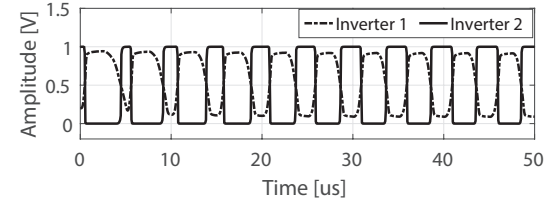
Fig. 4. Transient simulation showing how strings of non-changing data cause DC bias shifts which lead to pulse width expansion.
