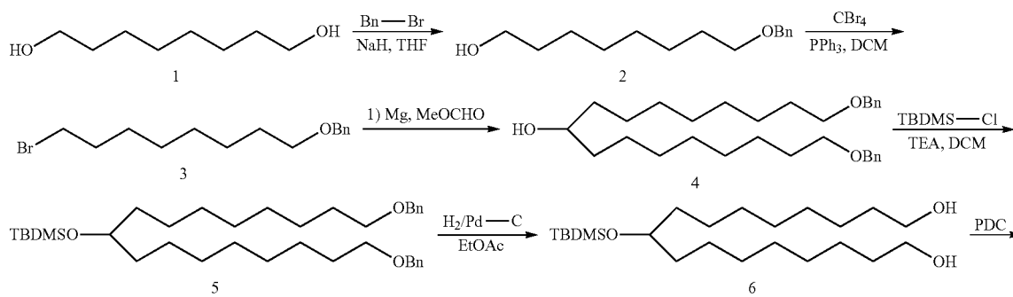
Scheme 20
