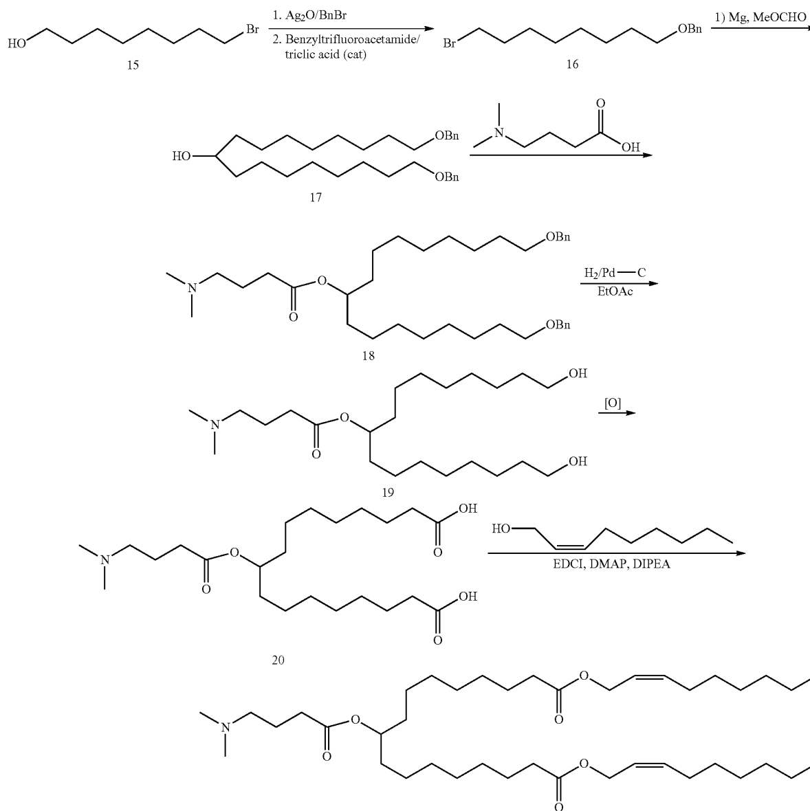
Scheme 19
