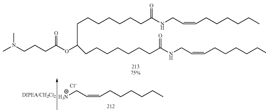
Scheme 11
