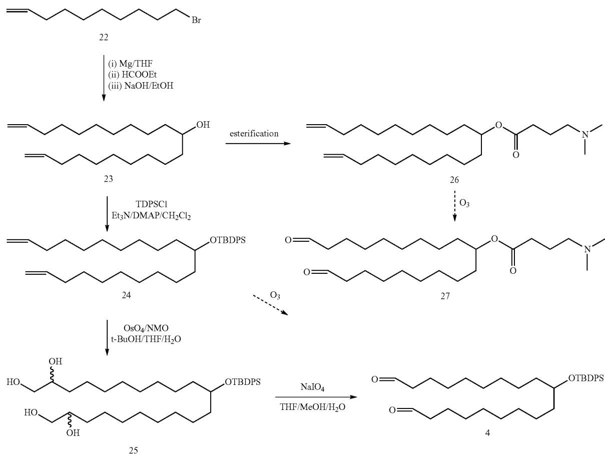
Scheme 3
