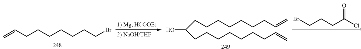
Scheme 18
