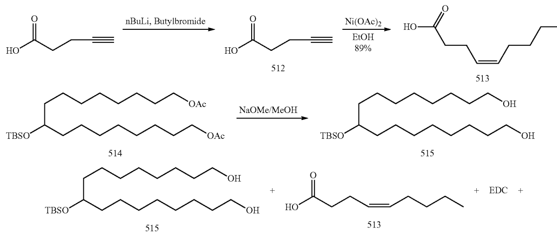
Scheme 26
