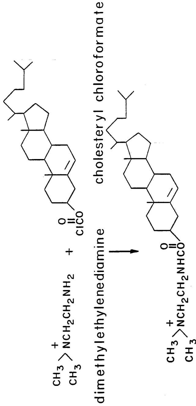
3β [N-(N',N'-dimethylaminoethane)-carbamoyl] cholesterol (DC-cho)
