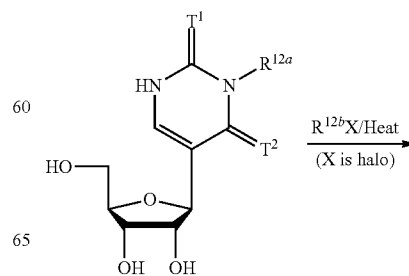
Scheme 11
