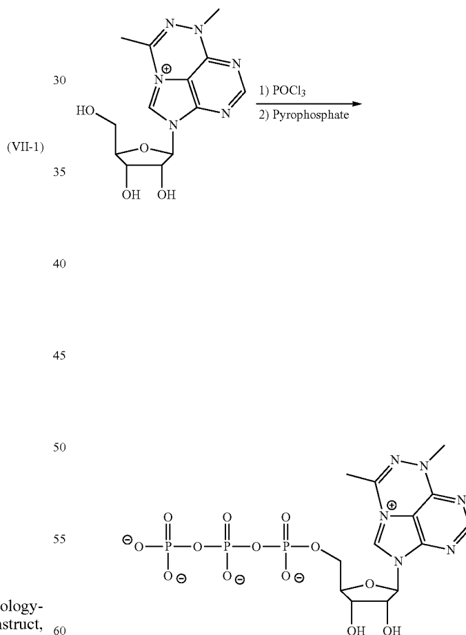
Scheme 1
