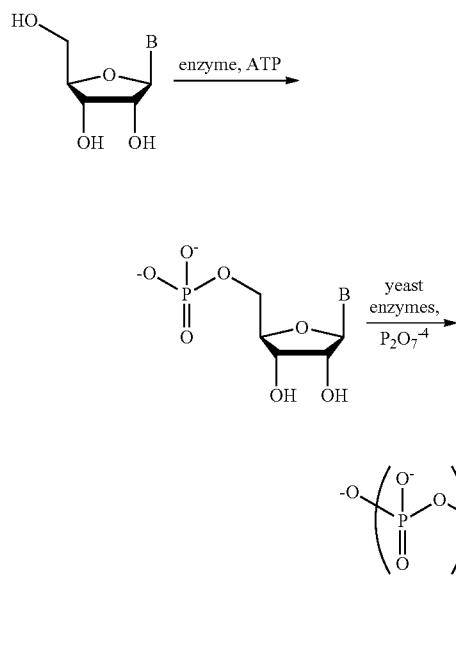
Scheme 10
