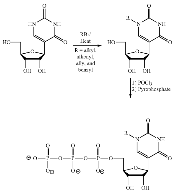
Scheme 5
