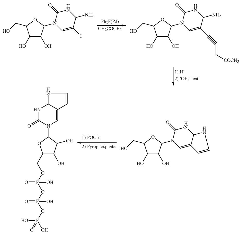
Scheme 9
