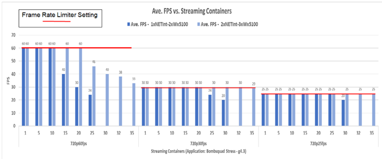
Figure 4: Game streaming - Anbox Cloud on eMAG with 2 vs 3 AMD WX5100 GPUs & 1 vs. 2 NETINT T408 video encoders
