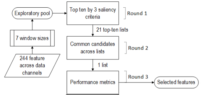
Figure 2. Feature selection process. 244 features as described in Table III. 7 window sizes are 2 \rightarrow 8 s in steps of 1 s. Three saliency criteria are DIS, MI, VarRatio scores. Common candidates are entries that are shared by more than one list of Round1 .
