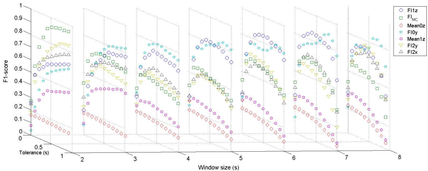
Figure 6. Effects of window sizes and tolerances on F1-scores of ASD. Tolerance from 0s \rightarrow 1 s. Three dimensional view for planes of window sizes from 2 s \rightarrow 8 s. Markers are for different features.
