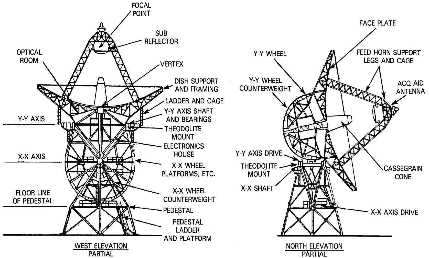
Figure 6-5. Deep Space Network 26-meter Antenna
