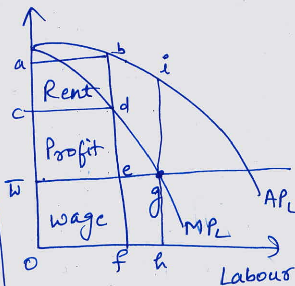
Fig 1 :- Ricardo Model
