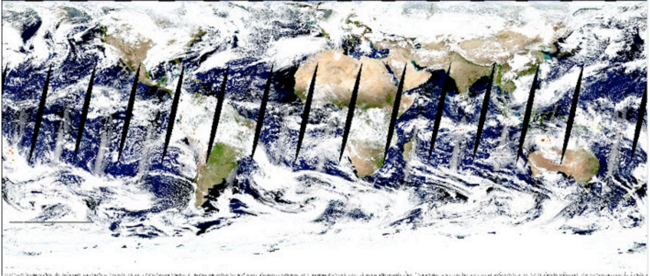
Figure 8. A MOD09CMG RGB-image composed of surface reflectance data measured by bands 1 (red), 4 (green) and 3 (blue) on December 7, 2000. The MODIS product granule ID is MOD09CMG.A2000341.005.2006347161131.hdf.
