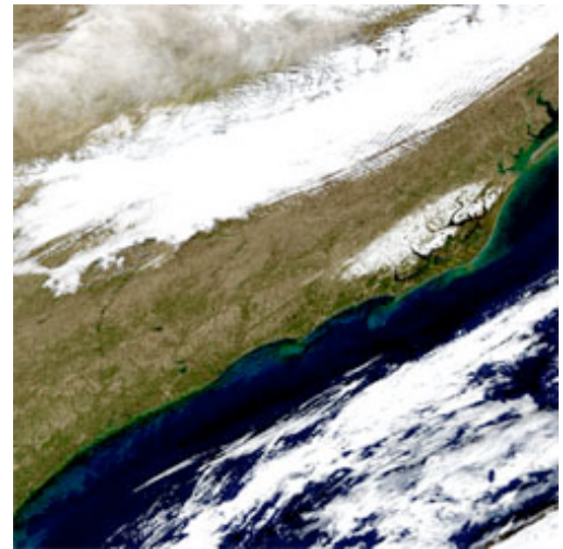
Figure 5. A MOD09GA RGB-image composed of surface reflectance measured by MODIS bands 1 (red), 4 (green) and 3 (blue) on December 6, 2000 over the US East coast. Product granule ID: MOD09GA.A2000340.h11v05.005.2006339102700.hdf
