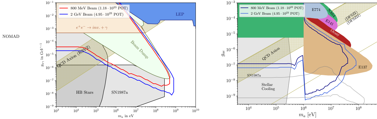
Fig. 29. Statistics-only, background-free, 90% C.L. sensitivity estimates for the axion-like particle (ALP) model. In five years of running, PIP2-BD can scan the g_{a\gamma} "cosmological triangle" region a large part of an untested parameter region for g_{ae} .
