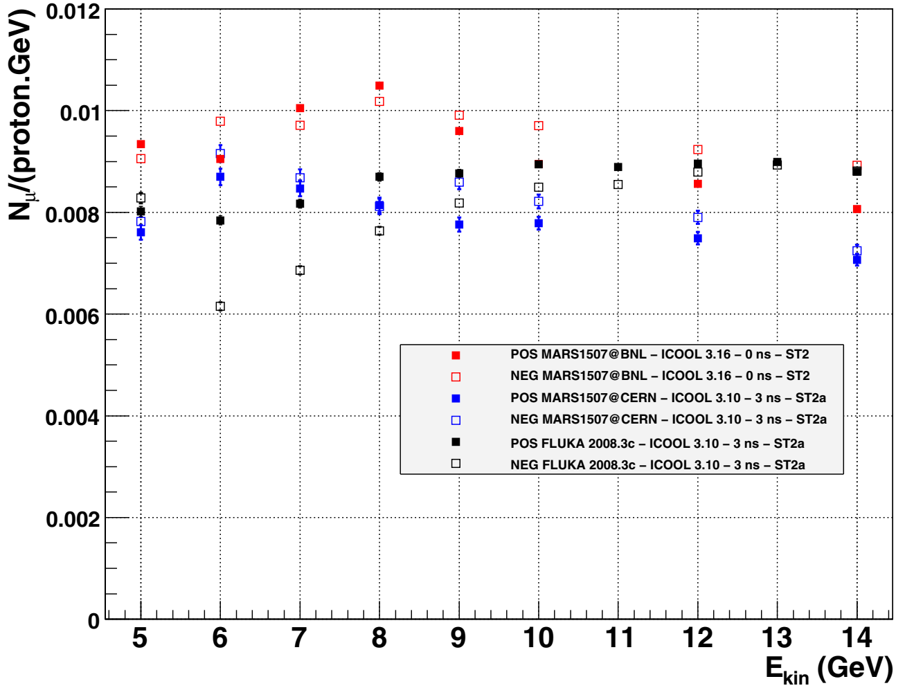
Figure 34. The muon yield, normalised to the beam power. An initial beam is generated by MARS as installed at BNL (red) and CERN (blue), and FLUKA 2008.3c (black), with an effective bunch length of 0 ns (red), 3 ns (blue and black). Mesons are then tracked through the front end using ICOOL 3.10 (blue) and ICOOL 3.16 (red). For the black points, an acceptance map approximating the effect of passing the particle through ICOOL 3.10 has been applied. After this, an acceptance cut is performed for a longitudinal momentum range of 100–400 MeV/ c , normalised longitudinal acceptance of 150 mm, and normalised transverse acceptance of 30 mm using ECALC9F [264]. ST2 and ST2a denote different field tapering parameters, with the field going from 20 T to 1.25 T and 1.75 T respectively.
