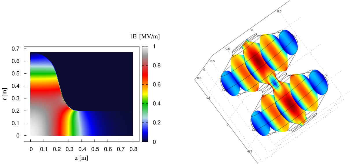
Figure 56. Main parameters of the superconducting RF cell and its electric field maps.
