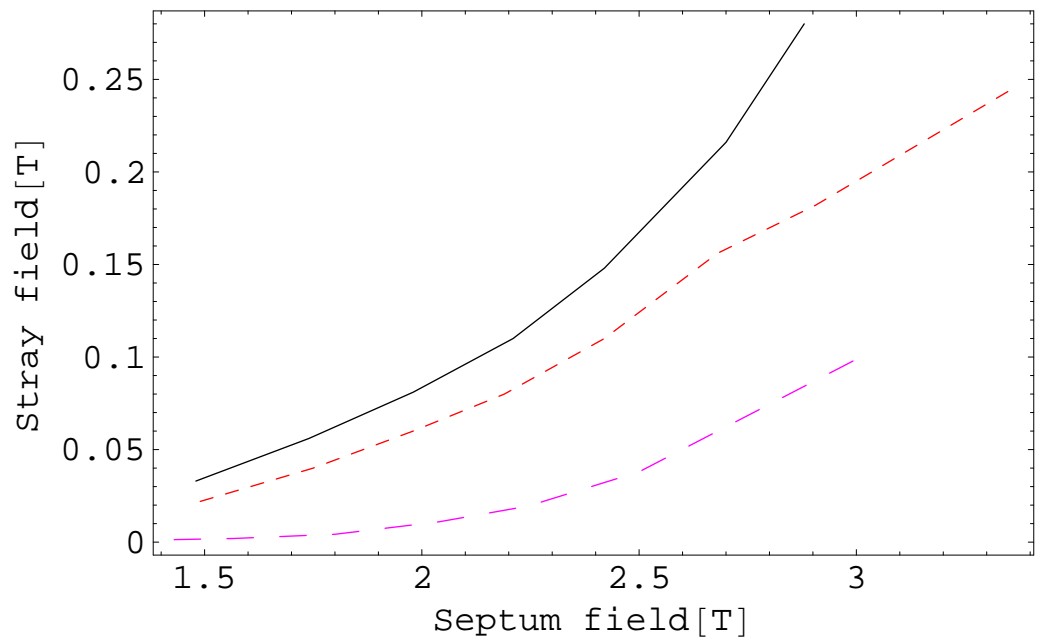
Figure 64. Stray fields in the superconducting septum using standard soft iron (black, solid line), using advanced material-VACOFLUX 50 (red line, short dash) and introducing a chamfer (magenta, long dash). The simulations were performed using the COMSOL 4.0 package.
