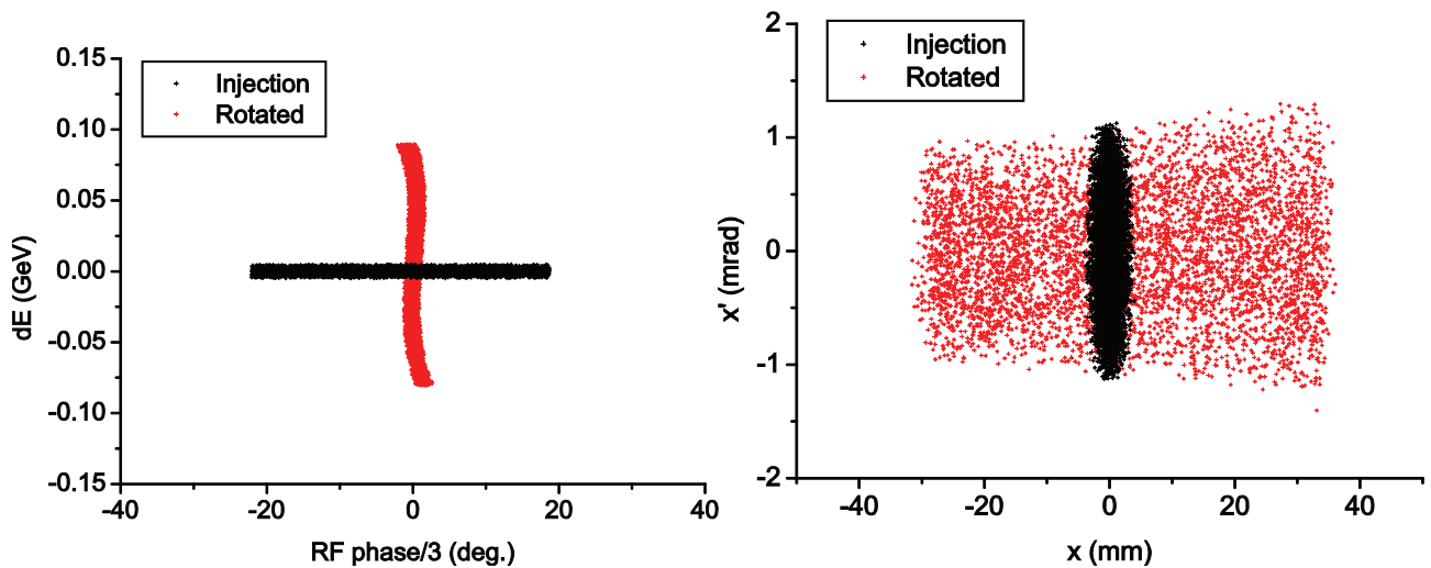
Figure 26. Phase space plots before and after bunch rotation.
