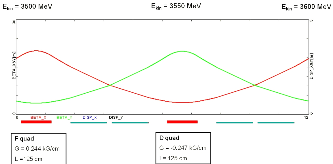
Figure 50. Periodic 90^\circ FODO linac cell (12 m), including two pairs of 2-cell cavities interleaved between quadrupoles.
