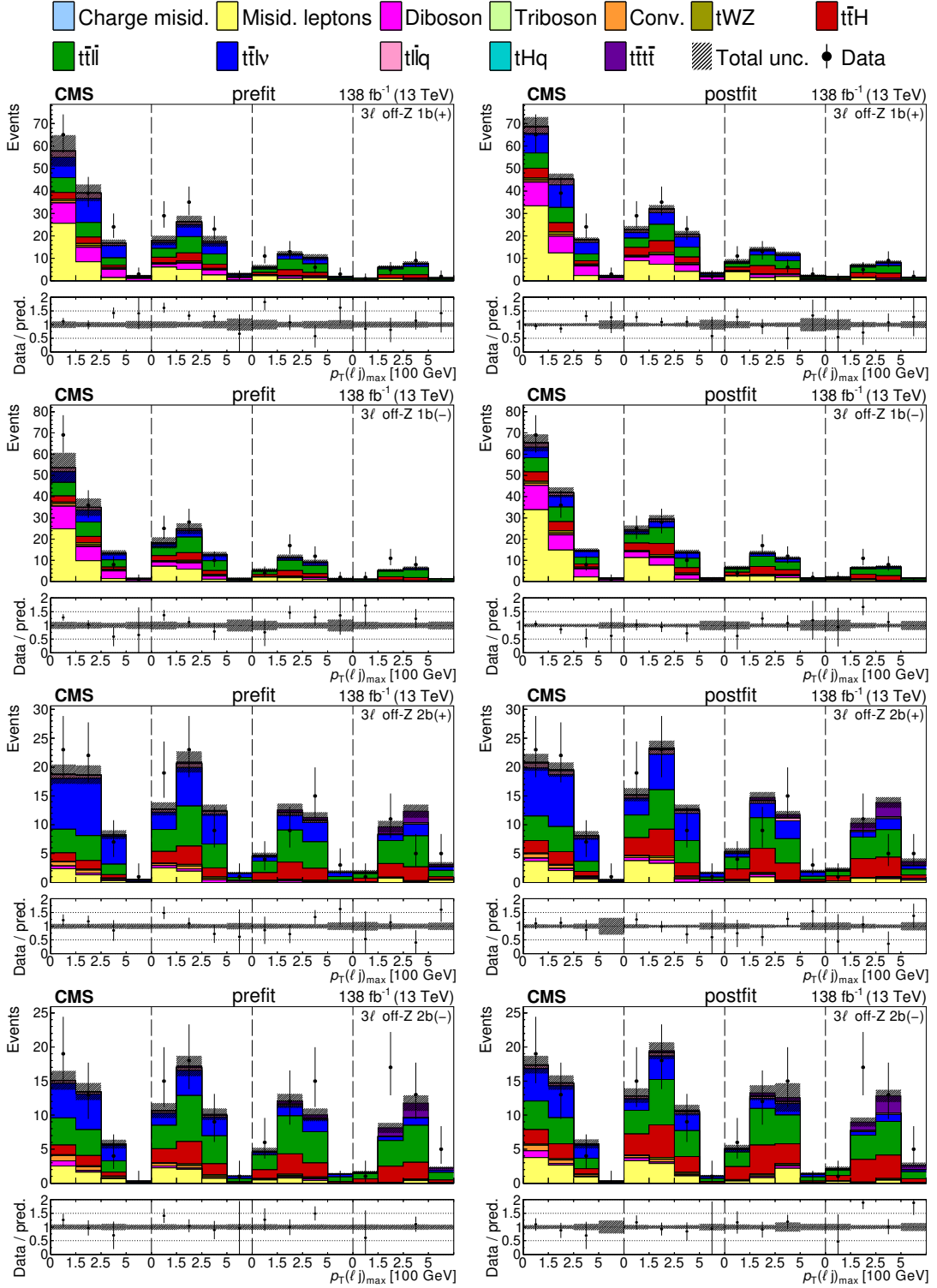
Figure 5: The categories shown in these plots are 3ℓ off-Z 1b and 3ℓ off-Z 2b. The prefit plots for each category are shown on the left side while the postfit plots are shown on the right side. The differential distribution in the plots is p_T(\ell)_{\max} . The jet subcategories are arranged from low jet multiplicity to high jet multiplicity from left to right for each individual plot. For example, in the 3ℓ off-Z 1b (+) plot, the first four bins are the p_T(\ell)_{\max} variable for 3ℓ off-Z 1b (+) 2j, the next four bins are for 3ℓ off-Z 1b (+) 3j, etc.
