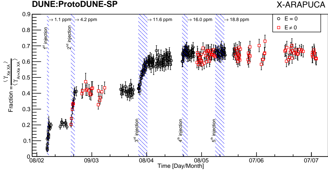
Figure 11: Fraction of light collected by the xenon-only sensitive X-ARAPUCA: \frac{\langle \gamma_{Xe} \rangle}{\langle \gamma_{Ar+Xe} \rangle} . The ratio increases with the doping and reaches a plateau around 0.65 for xenon concentration greater than 16.0 ppm. The red points correspond to data collected with the nominal TPC electric field, while black points refer to data with no electric field. Shaded areas indicate xenon injections.
