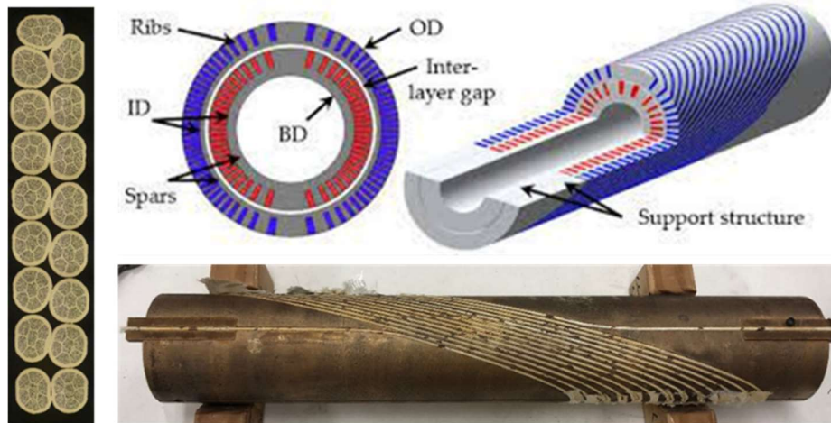
Fig. 14. BSCCO-2212 Rutherford cable (side left), CCT coil cross-section and 3D view (top right), and initial CCT BSCCO-2212 insert coil at LBNL (bottom right).
