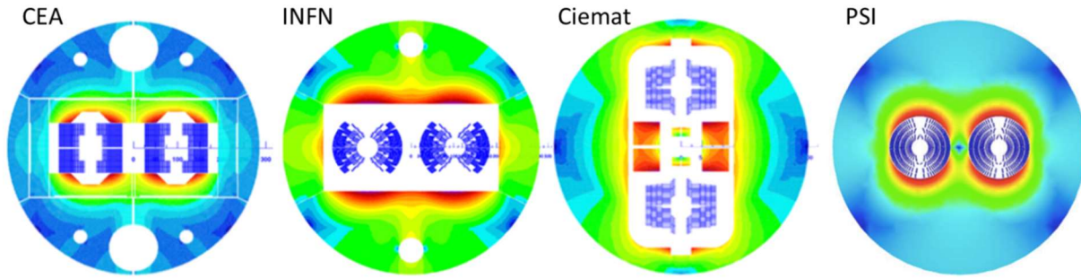
Fig. 6. FCC dipole conceptual designs (EuroCircol).
