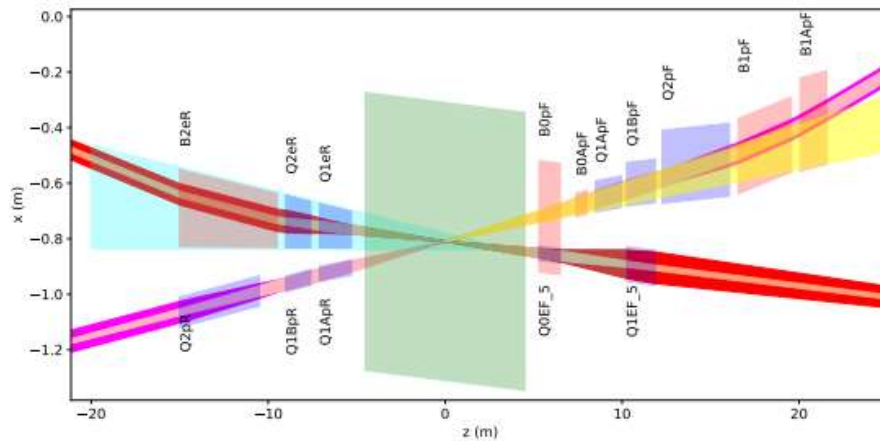
Fig. 4. IR1 layout. The central detector is shown in light green, the hadron and electron beams are shown in magenta and light red respectively. Magnet apertures are shown in light red for dipoles or light blue for quadrupoles. The forward neutron cone is shown in yellow.
