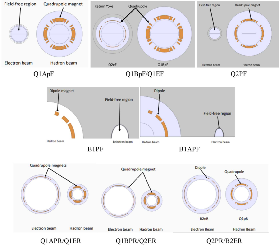
Fig. 5. Cross-sections of IR1 superconducting magnets.
