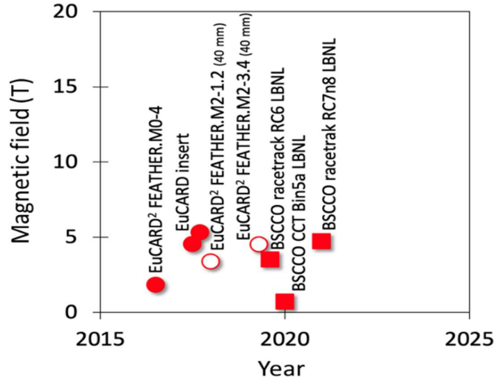
Fig. 12. Maximum fields obtained with demonstrator HTS short magnets, producing a transverse field of dipole type. All reported maximum value were reached in liquid helium (4.2 K). Solid symbols are coils with no bore (e.g., racetracks), while open symbols are real magnets, i.e., with a usable bore. Round symbols refer to coils built with REBCO, while square symbols refer to BSCCO-2212 coils.
