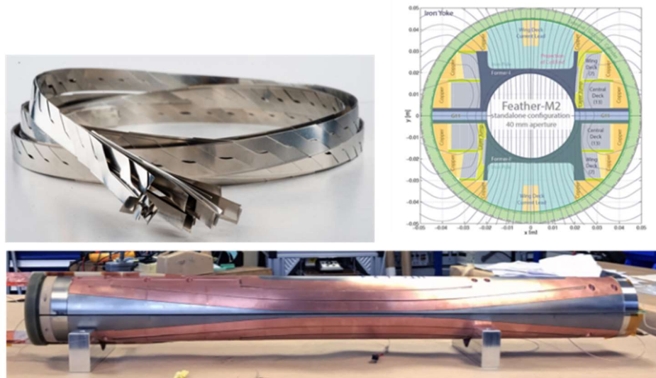
Fig. 13. EuCARD2 Roebel cable (top left), aligned block dipole sketch (top right), and first real insert coil before test at CERN (bottom).
