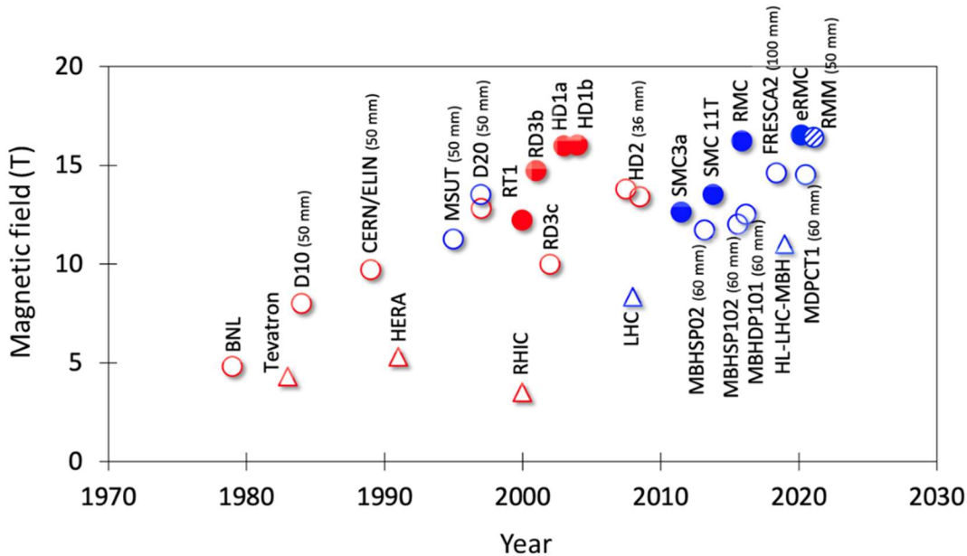
Fig. 10. Progression of fields reached by Nb 3 Sn dipole magnets of various configurations and dimensions. Open symbols represent magnets with a free bore, solid symbols are for demonstrators built with racetracks and no free bore. The hatched symbol (RMM) is a magnet with a free cavity. Tests were performed in liquid helium (4.2 K, red symbols) or superfluid helium (1.9 K, blue symbols). Superconducting collider dipole magnets are shown as triangles for comparison.
