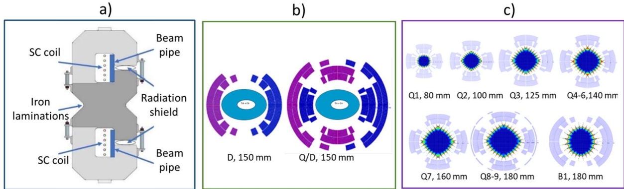
Fig. 9. MC acceleration and SR magnets: a) fast-cycling super-ferrie dipole magnet with HTS coil, b) collider dipole and combined function dipole-quadrupole magnets with thick elliptical absorbers in the apertures, c) IR quadrupole and dipole magnets (good field quality areas in the apertures are shown in blue color).
