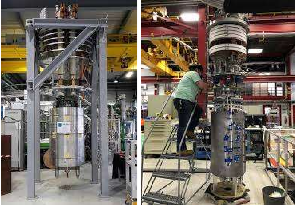
Fig. 11. The 14.6 T record dipole magnets: 100-mm aperture block-type FRESCA2 (left) and 60-mm aperture cos-theta MDPCT1.
