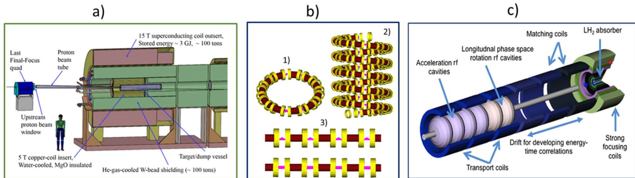
Fig. 8. MC solenoid concepts: a) muon production solenoid; b) various possible solenoid configurations in 6D muon cooling system; c) final cooling system with high-field solenoids.
