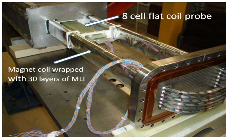
Fig. 18. Fast cycling dipole model based on REBCO tape.
