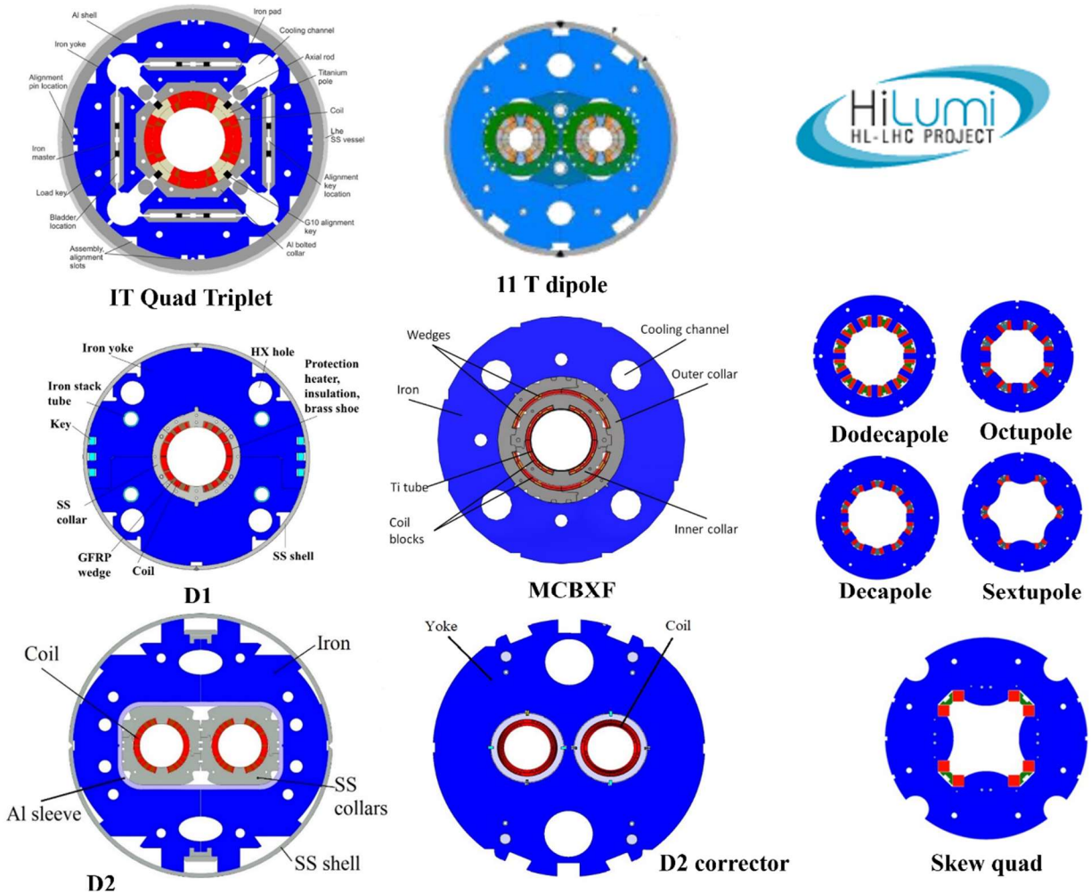
Fig. 2. The cross section of the various magnets developed for High Luminosity LHC.
