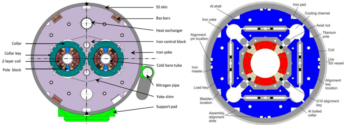
Fig. 3. Left: cross-section of the 11 T dipole cold mass. Right: cross-section of the MQXF cold mass. The two cross-sections are not in scale.
