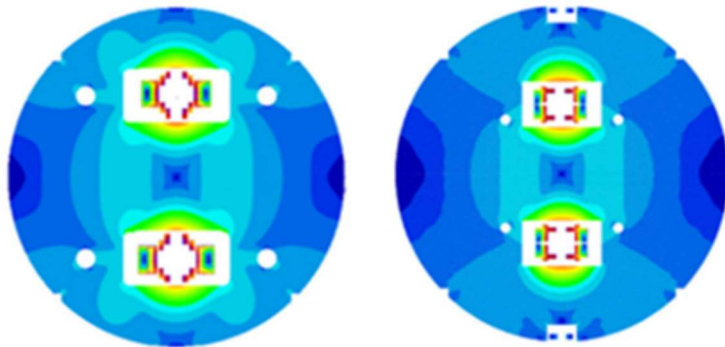
Fig. 7. Cross-sections of the two design options for the 12 T SPPC dipole based on IBS.
