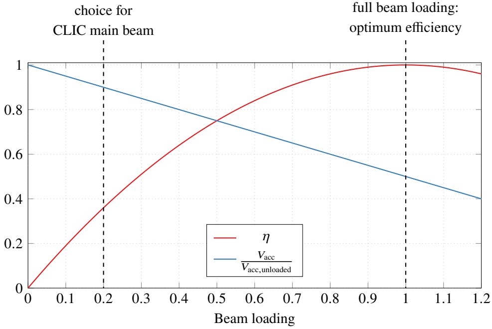
Figure 7.1. RF-to-beam power conversion efficiency ( \eta ) and accelerating voltage ( V_{acc} ) as a function of beam loading
