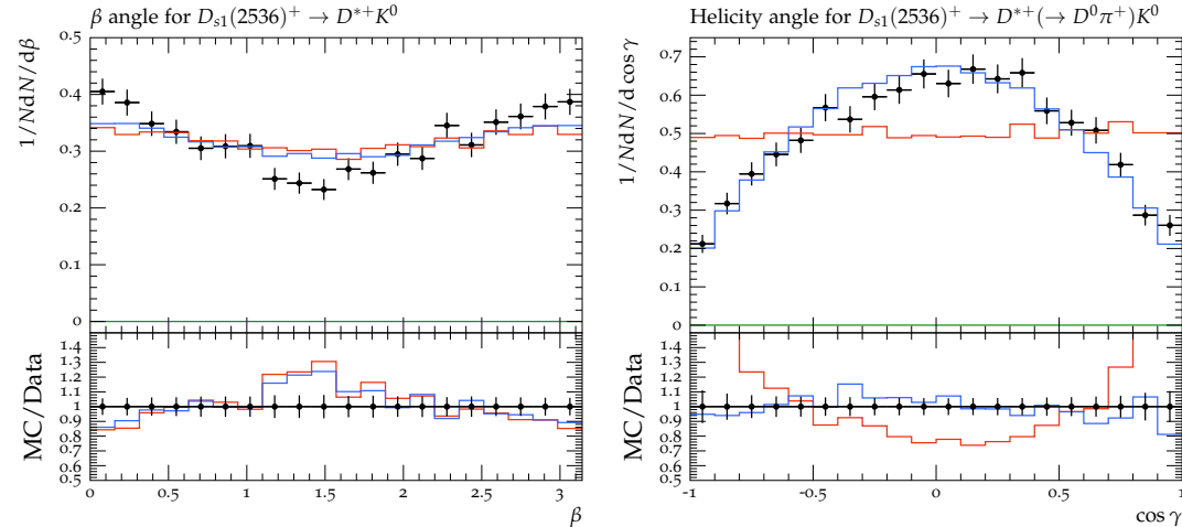
FIG. 9: Efficiency-corrected normalized signals as functions of \cos \gamma in comparison to experimental data from BELLE [1345]. Green Histograms show default predictions from HERWIG, while red and blue histograms are respectively predictions with only the implementation of HQEFT and with HQEFT effects in the presence of improved hadronization and decay models.
