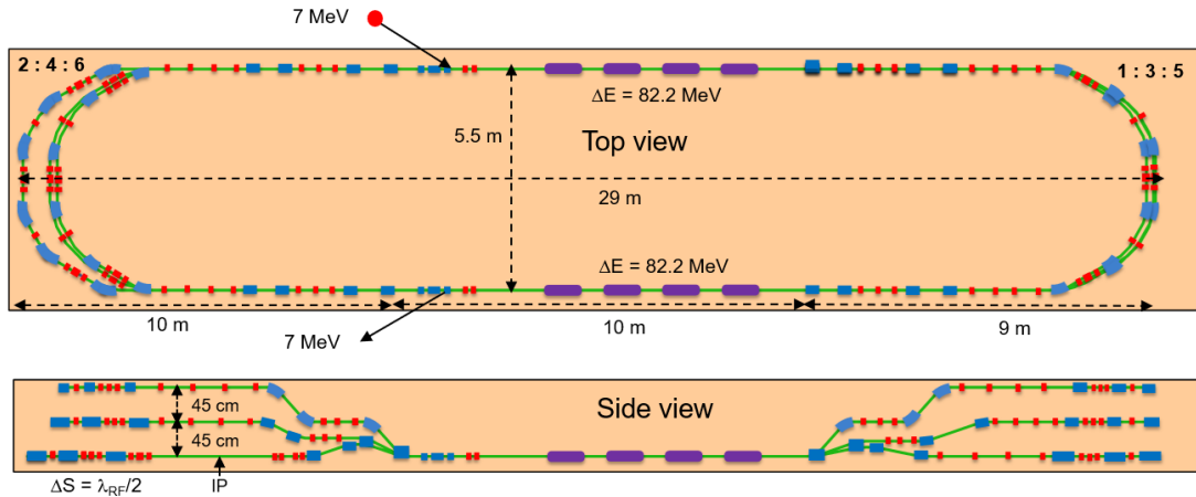
Fig. 6.3: Top and side views of the PERLE facility at IJCLab Orsay. An electron energy of 500 MeV is achieved in three turns passing through two cryomodules, each housing four 5-cell cavities of 802 MHz frequency. PERLE will be built in two stages, first with one linac cryomodule, adapted from the SPL module, and then completed with a newly designed one. The total number of magnets, including arcs, switchyards, merger and experiments, is 84 dipoles, 33 cm or 66 cm long, of typically 0.5 T to 1.0 T bend and 118 quadrupoles, 10 cm to 15 cm long, with fields of 0.4 kG/cm to 5.5 kG/cm.
