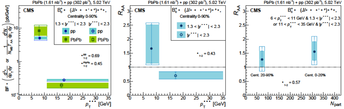
Figure 2: The B_c^+ meson production in pp and PbPb collisions. Left: The pp-equivalent cross-section times branching fraction of the studied decay in pp and PbPb collisions. Middle and right: The nuclear modification factor in p_T^{HMM} bins (middle), and in centrality bins integrated over the studied kinematic range (right). See the text for details.
