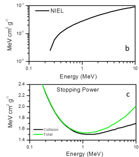
Figure 1-Top- NIEL curve evaluated with Electrons NIEL Calculator [13] for the Silicon with Exponential form factor and E_d=21 eV; Bottom- Collision and total stopping power for Si data reported in [14].
