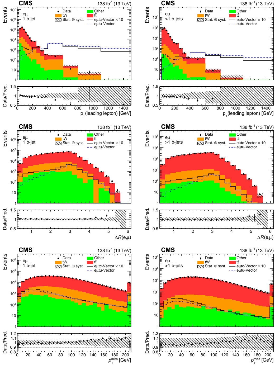
Figure 2: The distributions of the leading lepton p_T (upper row), \Delta R(e, \mu) (middle row), and p_T^{\text{miss}} (lower row) are shown for data (points) and simulation (histograms). Events with one or more b-tagged jets are shown in the left and right column, respectively. The hatched bands indicate the total uncertainty (statistical and systematic taken in quadrature) for the SM background predictions (cf. Section 6). Overflow events are added to the last bin. Examples of the predicted signal contribution for the vector type CLFV interactions via e\mu tu and e\mu tc vertices are shown, assuming C_x/\Lambda^2 = 1 \text{ TeV}^{-2} . The signal production- and decay-mode contributions are summed. The e\mu tc signal cross section is scaled up by a factor of 10 for improved visualization.
