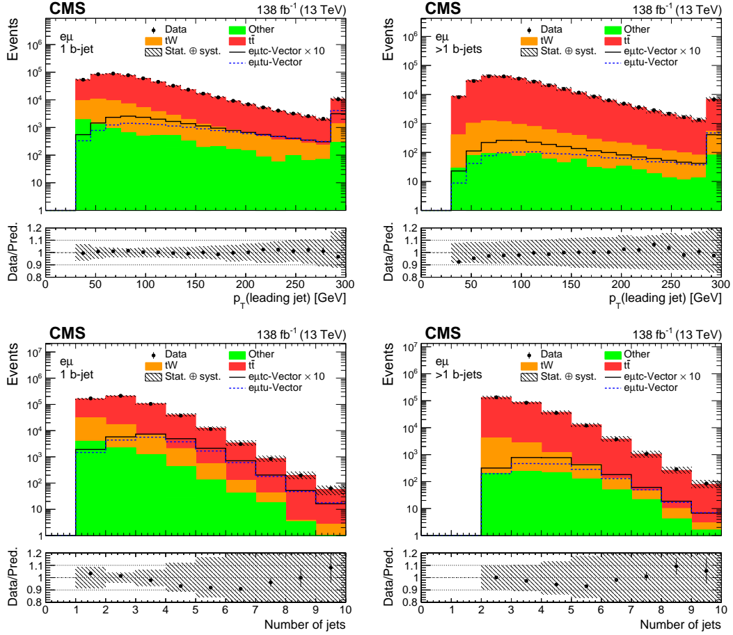
Figure 3: The distributions of the leading jet p_T (upper row) and the number of jets (lower row) are shown for data (points) and simulation (histograms). Events with one or more b-tagged jets are shown in the left and right column, respectively. The hatched bands indicate the total uncertainty (statistical and systematic taken in quadrature) for the SM background predictions (cf. Section 6). Overflow events are added to the last bin. Examples of the predicted signal contribution for the vector type CLFV interactions via e\mu tu and e\mu tc vertices are shown, assuming C_x/\Lambda^2 = 1 \text{ TeV}^{-2} . The signal production- and decay-mode contributions are summed. The e\mu tc signal cross section is scaled up by a factor of 10 for improved visualization.
