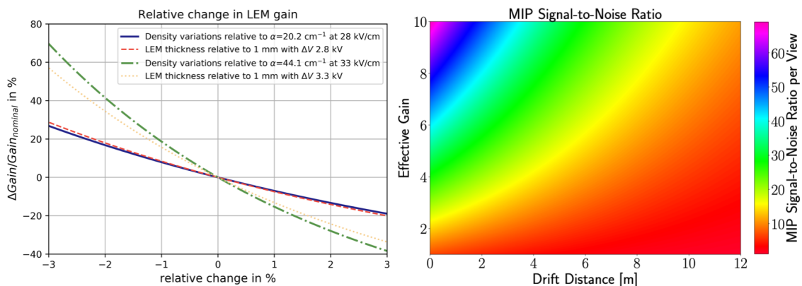
Figure 3. Left: relative fluctuation of \mathcal{G}_{LEM} around its nominal value when varying the gas density and LEM thickness from Table 1. The fluctuation is shown for two different values of E_{LEM} . Right: S/N from a MIP interaction collected per view on one anode strip as a function of the effective gain and drift distance. The S/N is computed for a MIP at an angle \varphi = 45^\circ , \theta = 90^\circ , purity of 75 [\text{O}_2]_{eq} ppt, drift field of 500 V/cm and noise of \text{ENC} = 2000 \text{ e}^- .
