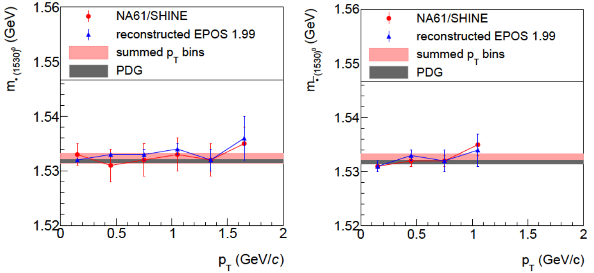
Figure 6: (Color online) Mass of \Xi(1530)^0 ( left panel ) and \bar{\Xi}(1530)^0 ( right panel ) fitted at mid-rapidity -0.25 < y < 0.25 as function of p_T for data (red points) and simulations (blue points). The red horizontal band presents the uncertainty of the fitted mass of \Xi(1530)^0 and \bar{\Xi}(1530)^0 using the events of the full data set (combining all y , p_T bins) and the grey bands the PDG values [6].
