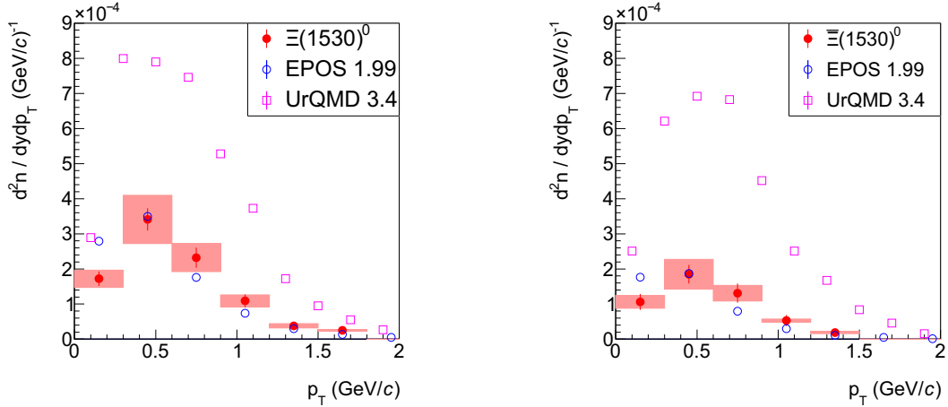
Figure 9: (Color online) Transverse momentum spectra at mid-rapidity of \Xi(1530)^0 (left) and \bar{\Xi}(1530)^0 (right) produced in inelastic p-p interactions at 158 \text{ GeV}/c . Shaded bands show systematic uncertainties. UrQMD 3.4 [14, 15] and EPOS 1.99 [13] predictions are shown as magenta and blue markers, respectively.
