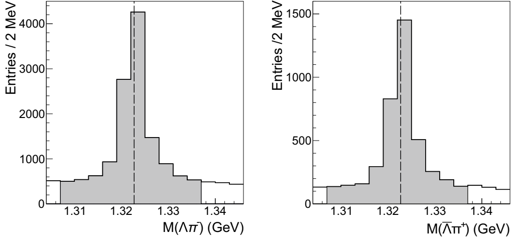
Figure 3: The (\bar{\Lambda}^+) invariant mass spectrum of (\bar{\Lambda}^+) candidates are shown in the left panel (right panel) . Filled areas indicate the mass range of the selected candidates. The vertical dashed black line shows the nominal PDG mass.
