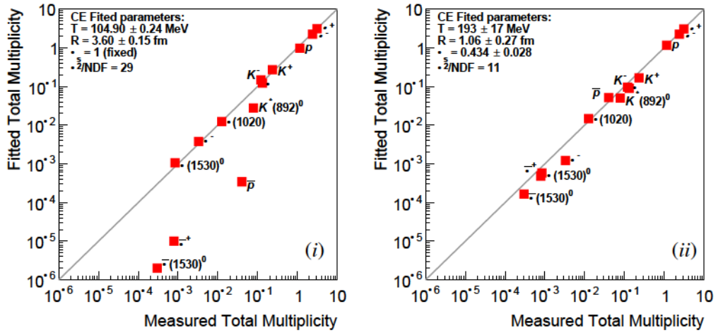
Figure 11: (Color online) Mean multiplicities of \pi^+ , \pi^- , K^+ , K^- , p , \bar{p} , K^*(892)^0 , \Lambda , \phi(1020) , \Xi^- , \Xi^+ , \Xi(1530)^0 and \Xi\bar{\Xi}(1530)^0 produced in p+p interactions at 158 GeV/c [3, 4, 17, 18, 19, 20, 12] measured by NA61/SHINE are compared with mean multiplicities obtained from the HRG model based on the Canonical Ensemble with fixed \gamma_s = 1 (i) and fitted \gamma_s (ii). Uncertainties of the measurements are smaller than the size of the markers.
