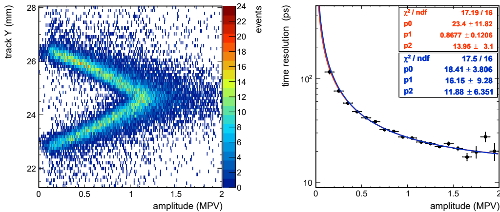
Figure 20: Left: Distribution of the signal amplitude, normalized to the MPV, for different impact point positions of the tracks along the y direction for a bar rotated by 45^\circ in the y plane; amplitudes decrease linearly with the crossed crystal thickness and therefore with the shift in the y direction from the impact point corresponding to the maximum crossing path length. Right: time resolution as a function of the amplitude of the signal in a 3 \times 3 \times 57 \text{ mm}^3 crystal bar coupled to HPK SiPMs. The dependence is shown for a discrimination threshold of 20 mV.
