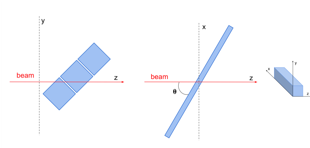
Figure 19: Sketch of the LYSO:Ce bars orientation with respect to the beam in two configurations: transverse cross section of the bars for a rotation in the y plane (left); rotation in the x plane with the beam forming an angle of incidence \theta with respect to the bar longitudinal axis (right).
