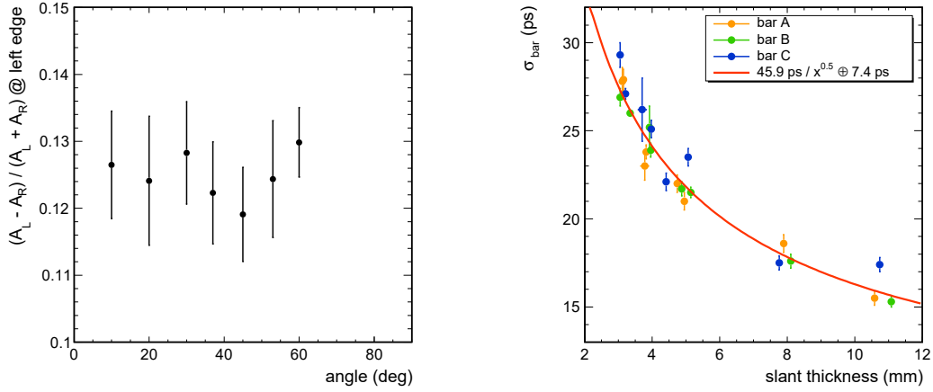
Figure 23: Left: asymmetry in the signal amplitude measured at the left and right SiPMs of a bar, defined as (A_L - A_R) / (A_L + A_R) @ left edge, as a function of the MIP impact angle. The asymmetry is estimated for tracks with impact point position at the left end of the bar. Right: time resolution of the individual bars in the three-bar array with HPK SiPMs as a function of the slant thickness obtained by tilting the setup by angles down to about 15° to the crystal axis. The slant thickness at each angle is estimated by scaling the crystal thickness (3 mm) by the ratio of the amplitude MPV at a given angle to the MPV at normal incidence.
