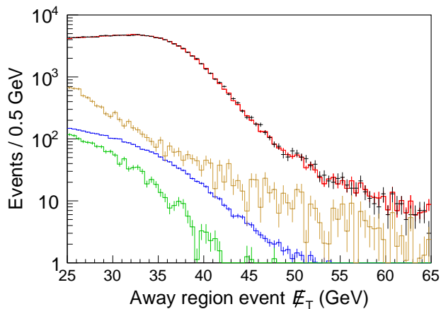
FIG. 14. E_T distributions for electron candidates in the plug calorimeter from the high-luminosity period, with n_{\text{vtx}} = 2 , and in the away region. The (black) crosses are the data and the (red) histogram overlapping the data is the simulation with all backgrounds. The backgrounds shown as examples from top to bottom are QCD (brown), \gamma^*/Z \rightarrow ee (blue), and W \rightarrow \tau\nu (green).
