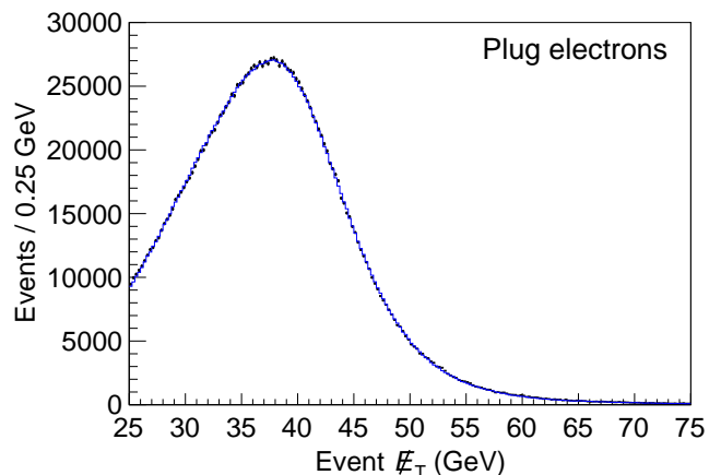
FIG. 11. Background-subtracted \cancel{E}_T distribution for electron candidates in the plug region. The crosses are the data and the solid histogram is the simulation. The comparison between the data and the simulation yields a \chi^2 of 310 per 200 bins.
