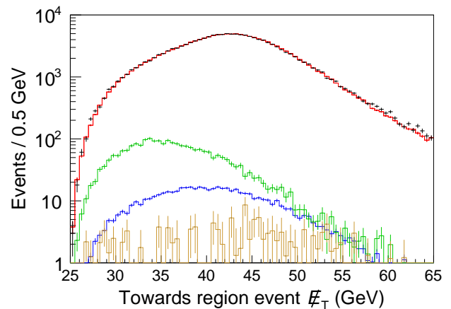
FIG. 16. E_T distributions for electron candidates in the plug calorimeter from the high-luminosity period, with n_{\text{vtx}} = 2 , and in the towards region. The (black) crosses are the data and the (red) histogram overlapping the data is the simulation with all backgrounds. The backgrounds shown as examples from top to bottom are W \rightarrow \tau\nu (green), \gamma^*/Z \rightarrow ee (blue), and QCD (brown).
