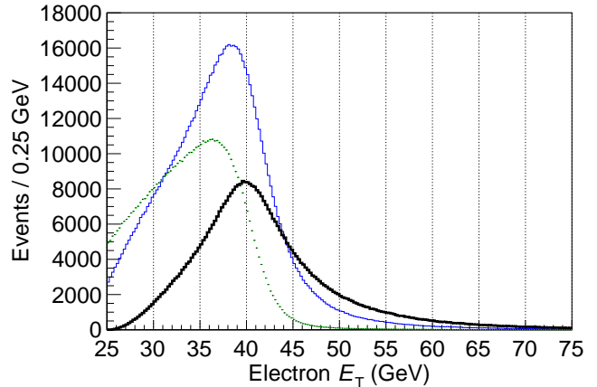
FIG. 5. Simulated E_T distributions of the away, transverse, and towards regions for the electrons in the plug calorimeter. Distributions for electrons in the central calorimeter are similar. The bold (black) histogram is for the away region, the light (blue) histogram is for the transverse region, and the (green) crosses are for the towards region. Corresponding E_T distributions follow a similar pattern except that away and towards are reversed because the direction away from the electron is towards the neutrino and vice versa.
