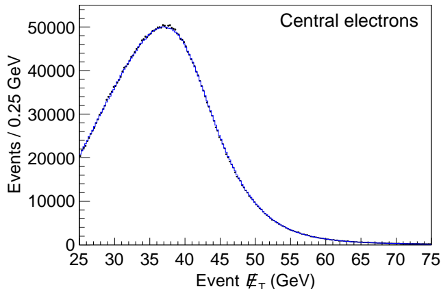
FIG. 10. Background-subtracted \cancel{E}_T distribution for electron candidates in the central region. The crosses are the data and the solid histogram is the simulation. The comparison between the data and the simulation yields a \chi^2 of 260 per 200 bins.
