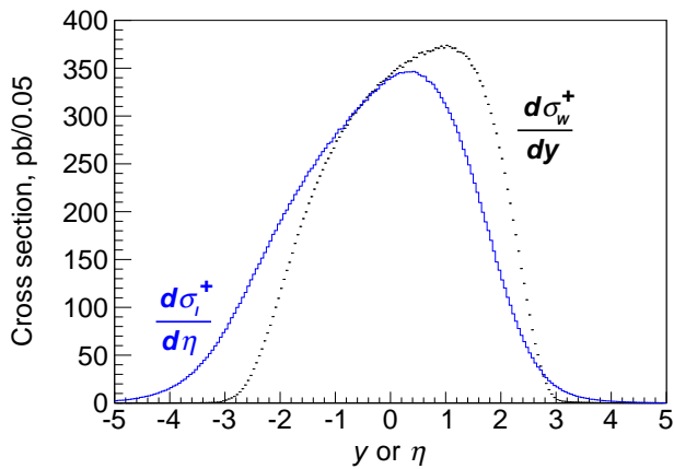
FIG. 2. d\sigma_W^+/dy and d\sigma_\ell^+/d\eta cross sections. The cross section for W^+ -boson ( W -decay charged-lepton) production in 1.96 TeV proton-antiproton collisions as a function of the rapidity (pseudorapidity). The cross sections are from the default calculation.
