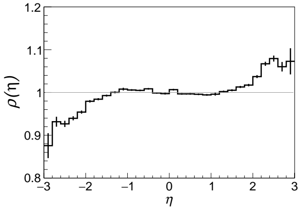
FIG. 4. The ratio \rho(\eta) (\epsilon A)^+ / (\epsilon A)^- as a function of \eta with the correct charge assigned to the reconstructed electrons. The uncertainties shown are statistical.
