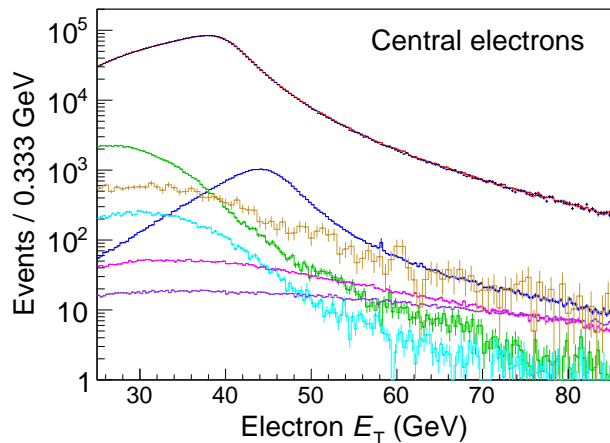
FIG. 17. E_T distributions of central-region electrons. The data are the crosses (black) and the simulation with all backgrounds is the histogram (red) overlapping the data. The individual backgrounds are the lower histograms, and from the top to bottom along the left edge of the plot they are the W \rightarrow \tau\nu (green), QCD (brown), \gamma^*/Z \rightarrow \tau^+\tau^- (cyan), \gamma^*/Z \rightarrow ee (blue), diboson (magenta), and t\bar{t} (purple) contributions.
