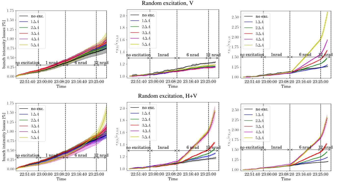
FIG. 19. Measured effects of the random excitation (in V, top row; and H+V, bottom row) during the 2017 experiment: relative intensity losses (left), relative horizontal emittance (center), and relative vertical emittance (right).
