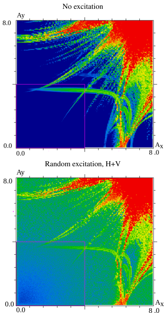
FIG. 17. FMA in transverse amplitude space without excitation (top) and with a random 1-nrad H+V excitation (bottom), based on the 2017 injection optics with no lattice errors and tunes (62.27, 60.295). Amplitudes are in units of \sigma .
