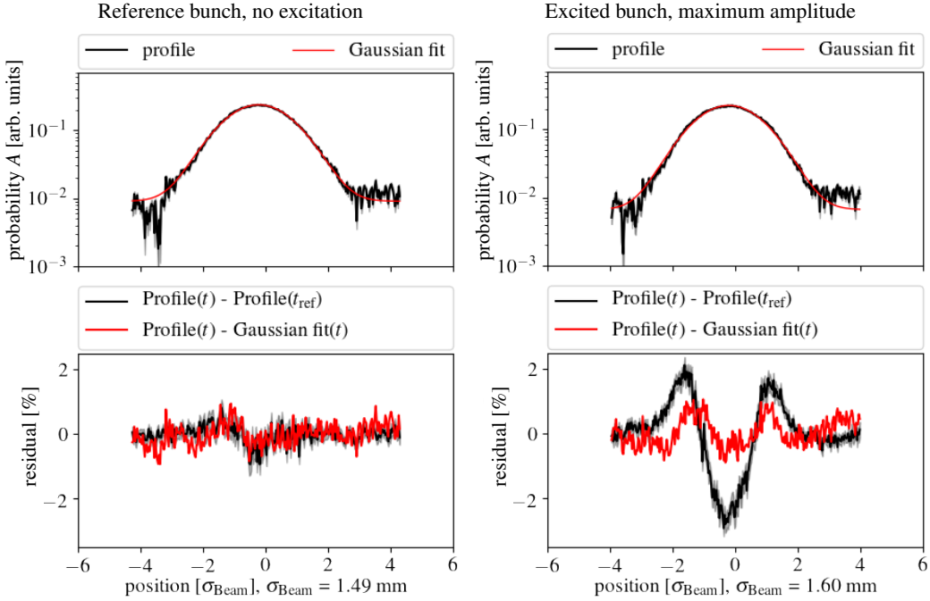
FIG. 11. Vertical beam profiles measured with the Beam Synchrotron Radiation Telescope (BSRT) during the 2016 experiments on 10th-turn pulsing in the vertical plane. The transverse damping system was not active on these bunches. The beam distributions at the end of the excitation period are shown in black in the top plots, with a Gaussian fit in red. The bottom plots show the residuals: final profile minus initial profile (black); final profile minus its Gaussian fit (red). Residuals are expressed as a fraction of the peak profile amplitude. The black lines in the plots of the residuals are a measure of the overall change of the distribution shape. The red lines indicate how different the final distributions are from a Gaussian shape. Details of the analysis are given in Ref. [35]. The distribution of the reference bunch (left) is almost unchanged, whereas the bunch experiencing the maximum excitation (right) shows a clear shift of particles from the axis towards approximately \pm 2\sigma .
