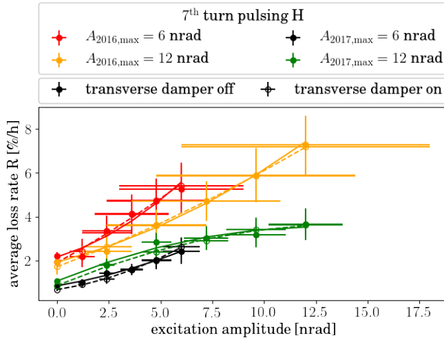
FIG. 15. Measured loss rates vs. excitation amplitude for 7th-turn pulsing in the horizontal plane during the 2016 experiment (red and yellow) and the 2017 experiment (black and green). In 2017, horizontal, vertical and combined pulsing had similar effects [13]. The uncertainties on the excitation amplitude are dominated by the calibration of the transverse feedback and damping system. The uncertainties on the loss rates are statistical. An estimate of the systematic uncertainties (due to changes in beam distribution, for instance) is given by the difference between the two data sets within each experiment. The lines indicate empirical second-order polynomial fits, with damper off (solid) and with damper on (dashed).
