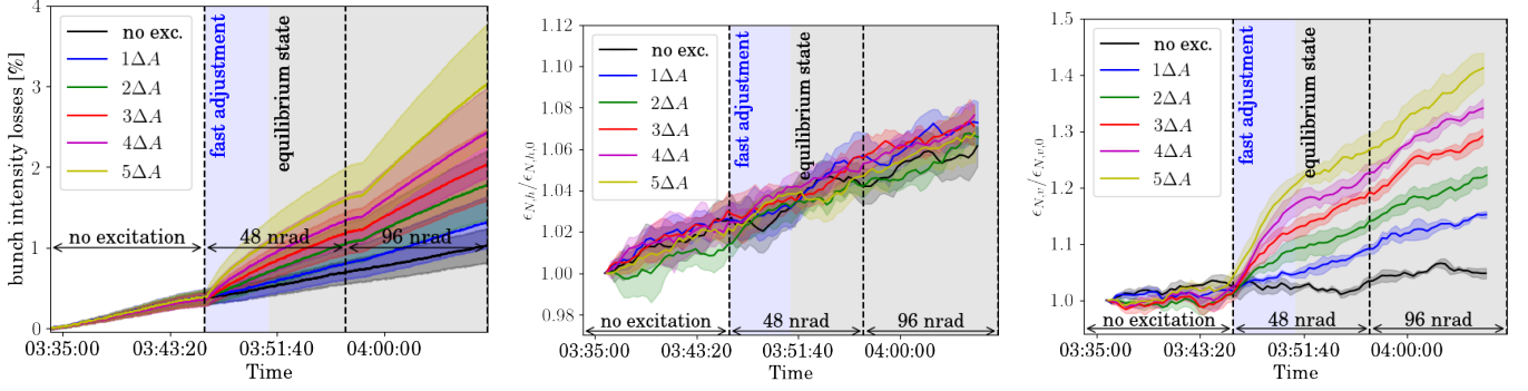
FIG. 10. Summary of the 2016 experiments on 10th-turn pulsing in the vertical plane: losses (left), horizontal emittances (middle) and vertical emittances (right), relative to their initial values. The transverse damping system was not active in this case. The 3 excitation periods are labeled in black according to the value of the maximum excitation amplitude A_{\max} = 5\Delta A : no excitation, 48 nrad or 96 nrad. The 4 bunches experiencing the same excitation amplitude n\Delta A ( n = 0, \dots, 5 ) are grouped by color. The data are averaged over the 4 bunches, with the envelope representing the standard deviation. The area with a blue background highlights qualitatively the fast adjustment period of the beam distribution, transitioning into a new equilibrium state (indicated by the gray background).
