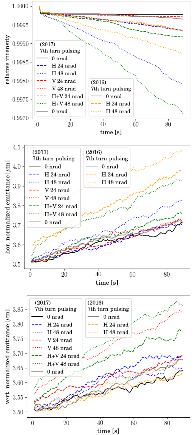
FIG. 13. Calculated bunch intensities and emittances from distribution tracking based on the 2016 injection optics with standard lattice errors and (Q_x, Q_y) = (64.28, 59.31) and 2017 injection optics with standard lattice errors and (Q_x, Q_y) = (62.27, 60.295) : relative intensity (top); horizontal emittance (middle); vertical emittance (bottom). The solid black line includes only a random dipole noise component in H+V of 6 nrad. The dotted and dashed lines correspond to 7th-turn pulsing with two different excitation amplitudes (24 nrad and 48 nrad), plus a random dipole noise component in H+V of 6 nrad.
