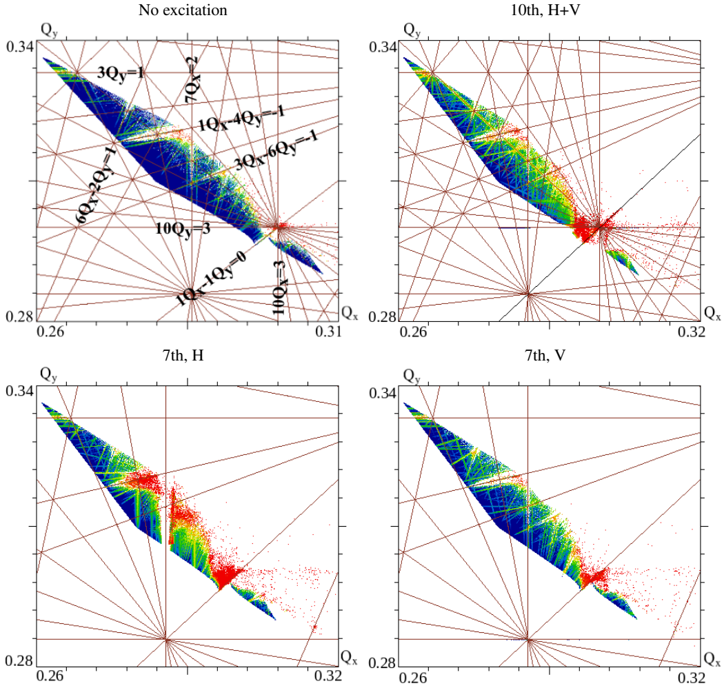
FIG. 8. Frequency-map analysis in betatron tune space based on the 2016 injection optics with no machine errors and tunes (64.28, 59.31): without excitation (top left); 10th-turn pulsing in both horizontal and vertical planes (top right); 7th-turn pulsing in the horizontal (bottom left) and vertical (bottom right) planes. The excitation amplitude is 120 nrad in the corresponding plane. The colors (blue to red) represent the tune jitter of tracked particles starting at each given location in tune space [39]. The absence of a strong excitation of any resonance in case of vertical 7th-turn pulsing and the strong excitation in case of horizontal pulsing confirms the excitation of the 7Q_x resonance. For 10th-turn pulsing, there is in contrast no significant difference between H, V, or H+V [13].
