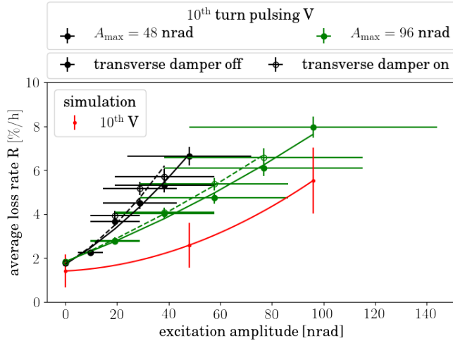
FIG. 12. Comparison between experiments and simulations of loss rates vs. resonant excitation amplitude for 10th-turn pulsing in the vertical plane. The relative average loss rate R is defined in Eq. 14. The experimental results for a maximum excitation amplitude of 48 nrad are shown in black and those for 96 nrad are plotted in green (see also Fig. 10, left, for instance). The results with damper off are represented by solid dots, those with damper on are shown with open circles. The simulation results, including random dipole noise, are shown in red [13]. Statistical and systematic uncertainties are discussed in the text. The curves represent empirical quadratic fits to the data with damper off (solid) and with damper on (dashed).
