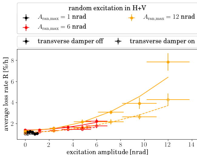
FIG. 20. Measured loss rates as a function of amplitude for random excitations in H+V. Three consecutive data sets were taken (black, red, and yellow), with increasing maximum amplitude. Data were taken simultaneously with no transverse damper on some bunches (filled circles and solid lines) and with the damper active on other bunches (empty circles and dashed lines). The lines represent empirical second-order polynomial fits.
