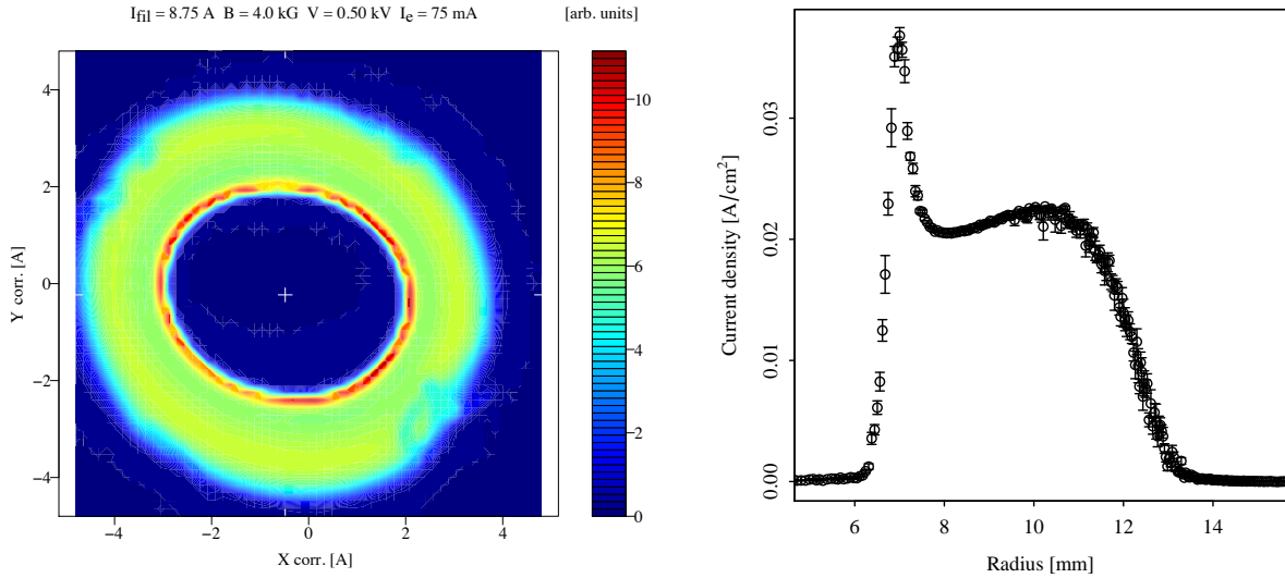
FIG. 4. Example of current-density distribution measurements for the hollow electron gun prototype CHG1b, taken at the Fermilab electron lens test stand in 2017 [26]: 2-dimensional transverse profile measurement (left) and calculated 1-dimensional radial projection (right).
