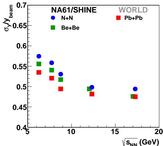
Figure 16: Collision energy dependence of the ratio of the width \sigma_y of the rapidity distribution to the beam rapidity y_{beam} for central Be+Be and Pb+Pb collisions and inelastic N+N interactions.
