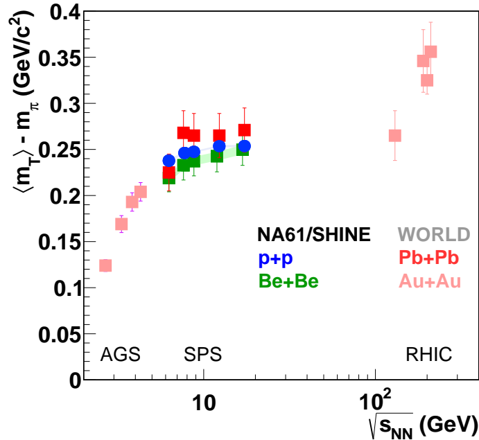
Figure 17: Energy dependence of the mean transverse mass of \pi^- measured at mid-rapidity in central Be+Be, Pb+Pb [2, 3] and Au+Au [32, 33] collisions and inelastic p+p interactions [34].
