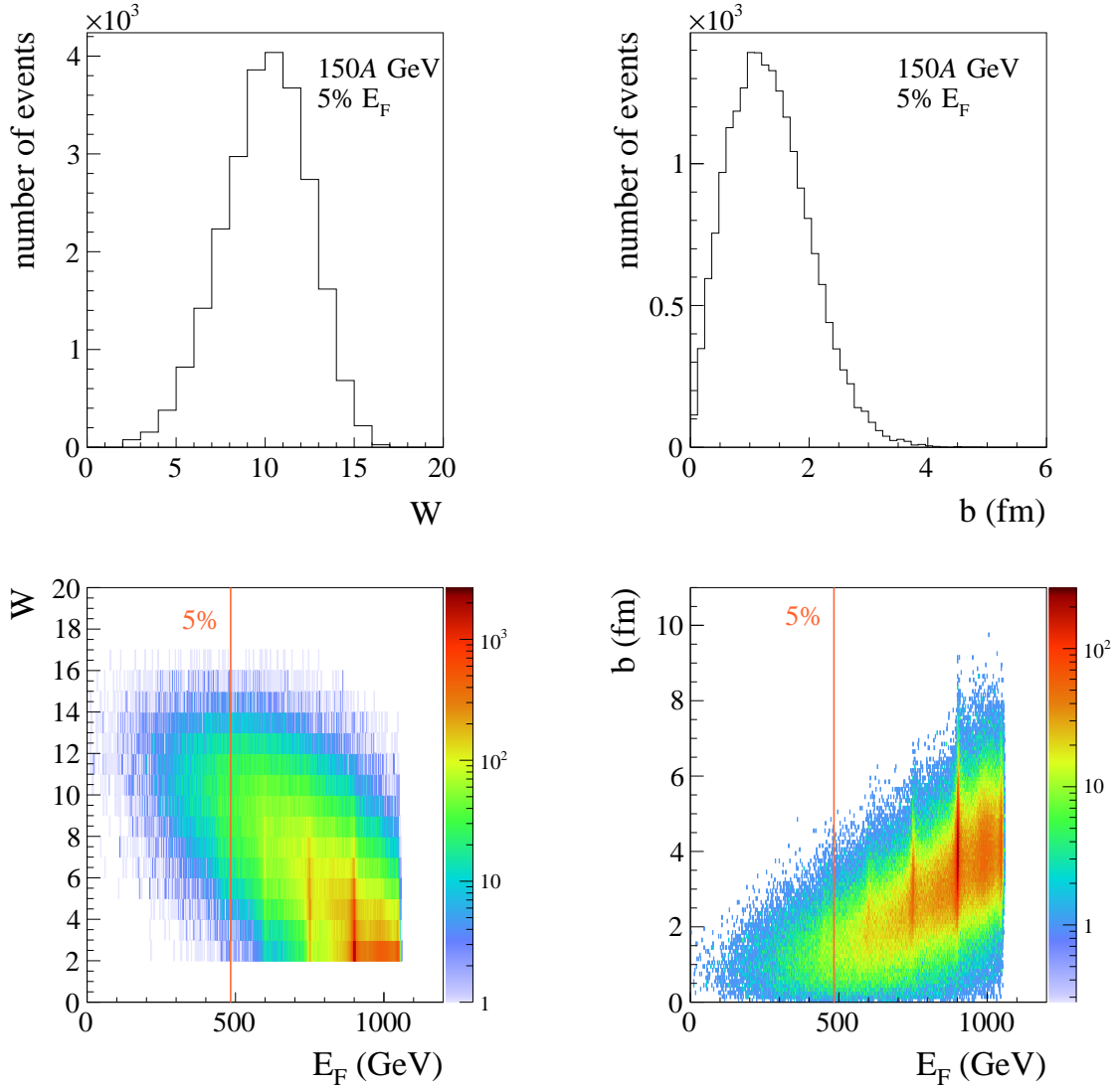
Figure 7: Examples of the distribution of the number of wounded nucleons W ( top, left ) and impact parameter b ( top, right ) for events with the 5% smallest forward energies E_F and E_F versus W ( bottom, left ) and E_F versus b ( bottom, right ) at beam momentum of 150A GeV/ c simulated with EPOS using the acceptance map provided in Ref. [21].
