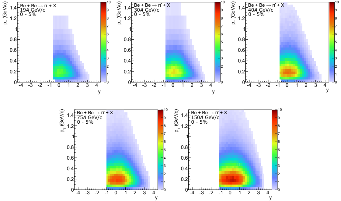
Figure 9: Double-differential spectra \frac{d^2n}{dydp_T} of negatively charged pions produced in the 5% most central Be+Be collisions at beam momenta of 19A, 30A, 40A, 75A and 150A GeV/c.
