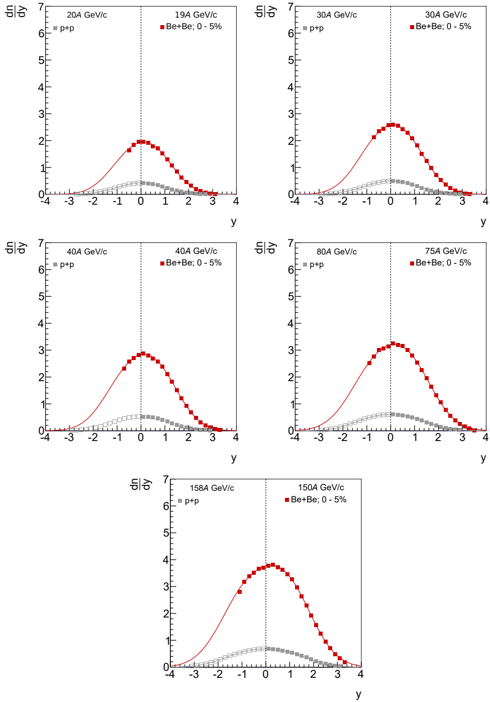
Figure 15: Rapidity spectra of \pi^- produced in the 5% most central Be+Be collisions at the SPS energies. Results from inelastic p+p interactions [12] are shown for comparison. Statistical errors are smaller than the size of the markers.
