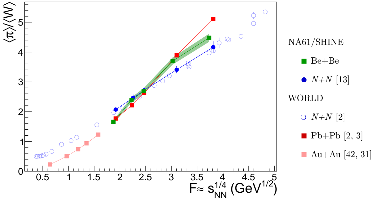
Figure 19: The "kink" plot showing the ratio of pion multiplicity \langle\pi\rangle to number of wounded nucleons \langle W\rangle versus the Fermi energy variable F \approx s_{NN}^{1/4} . Results from central Be+Be collisions are compared to measurements in for inelastic nucleon-nucleon reactions and central collisions of heavier nuclei. Results of Be+Be collisions are shown with statistical (vertical lines) and systematic (shaded band) uncertainties. All other results are presented with total uncertainty.
