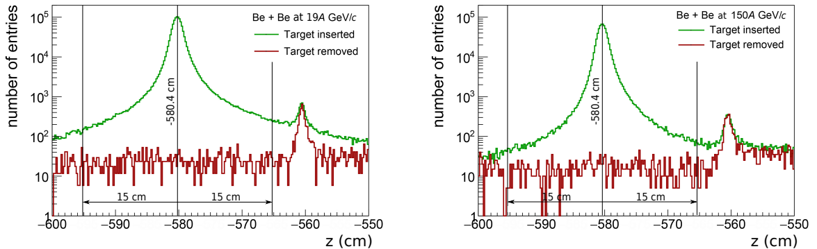
Figure 8: Distribution of fitted vertex z coordinate for the 20% most central {}^7\text{Be}+{}^9\text{Be} interactions with target inserted (green histogram) and target removed (red histogram). ( Left ): 19A GeV/ c . ( Right ): 150A GeV/ c . Target position and cut values are marked. Target is installed in the box filled with He gas to minimise background interactions. Smaller peak on the right hand side of the plots corresponds to interactions with a target holder window.
