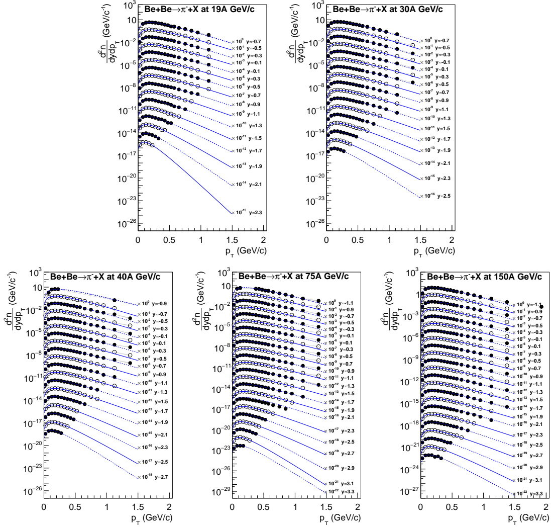
Figure 10: Transverse momentum spectra of \pi^- in rapidity slices produced in the 5% most central Be+Be collisions. Rapidity values given in the legends correspond to the middle of the corresponding interval. Data points for consecutive rapidity slices are scaled down by factors of 10. Shaded bands show systematic uncertainties. Curves depict thermal model motivated fits with Eq. 4.
