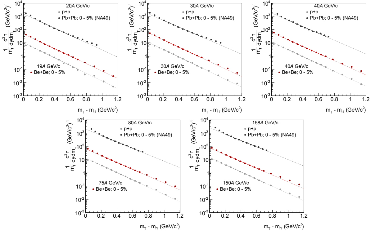
Figure 12: Transverse mass spectra \frac{1}{m_T} \frac{d^2n}{dy dm_T} of negatively charged pions produced in central Be+Be collisions at the SPS energies. Statistical errors are smaller than the size of the points. Results from inelastic p+p interactions [12] and central Pb+Pb interactions [2, 3] are shown for comparison. Lines show exponential fits with Eq. 4.
