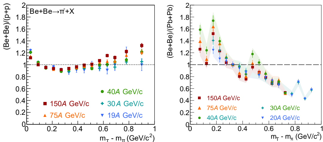
Figure 13: Ratio of normalized transverse mass spectra: Be+Be/ p+p (left) and Be+Be/Pb+Pb (right) at the SPS energies.
