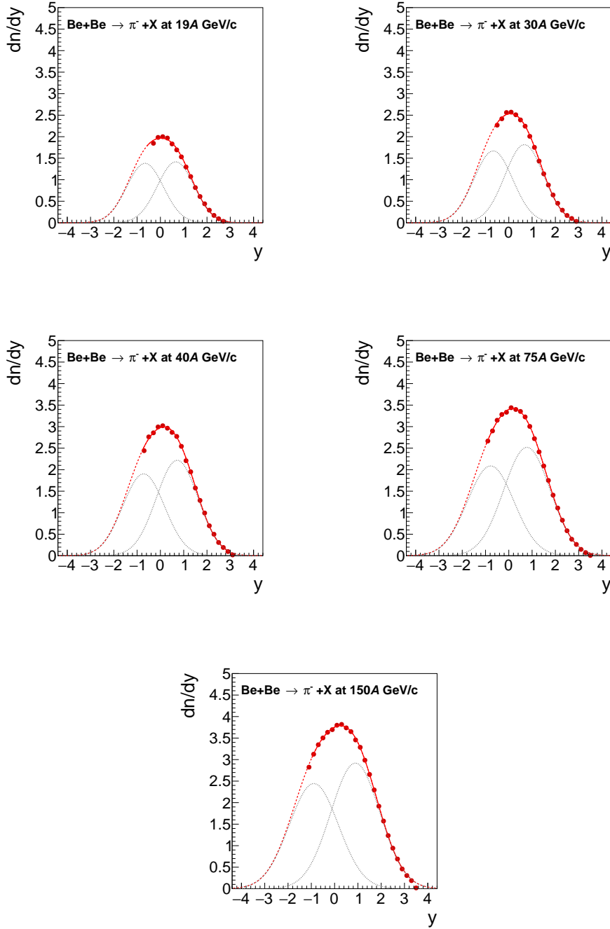
Figure 14: Rapidity distributions of negatively charged pions in central Be+Be collisions at the SPS energies. The parametrization of the spectra by Eq. 5 is shown. The solid line shows the fitted function in the range of the fit, and the red dashed line depicts the extrapolation of the fitted function. The two Gaussian functions constituting the fitted function are represented by the black dashed lines.
