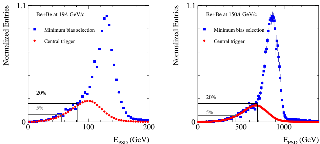
Figure 6: Two examples of the measured E_{PSD} distribution for minimum-bias selected (blue data points) and T2 selected (red data points) events at 19A GeV/c ( left ) and 150A GeV/c ( right ) beam momentum. Histograms are normalized to agree in the overlap region. The limits used to select events are shown by black lines and they correspond to \approx 5\% and \approx 20\% of inelastic collisions.
