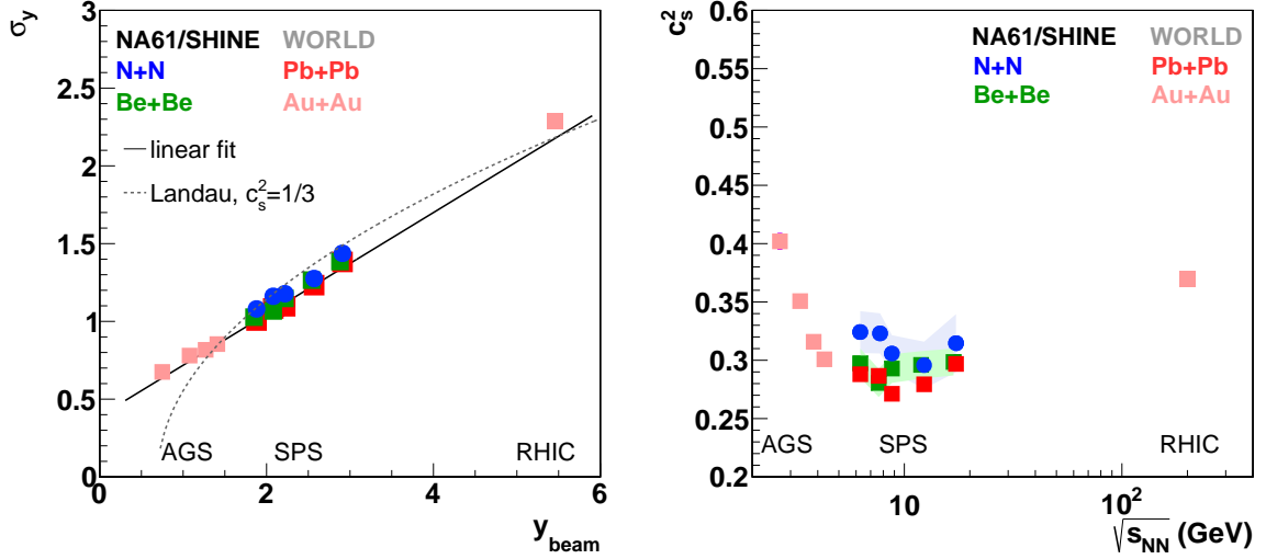
Figure 18: Comparison of the Landau hydrodynamical model with rapidity distributions of charged pions produced in central nucleus-nucleus collisions and inelastic nucleon-nucleon interactions. Left: The width \sigma_y of the rapidity distributions of negatively charged pions in central Be+Be, Pb+Pb [2, 3] (Au+Au [32, 33]) reactions and the width \sigma_y of the average of rapidity distributions of positively and negatively charged pions in p+p [13, 34] (denoted as N+N ) as a function of the beam rapidity y_{beam} . The dotted line indicates the Landau model prediction with c_s^2 = 1/3 , while the full line shows a linear fit through the data points. Right: The speed of sound as a function of beam energy as extracted from the data using Eq. 7.
