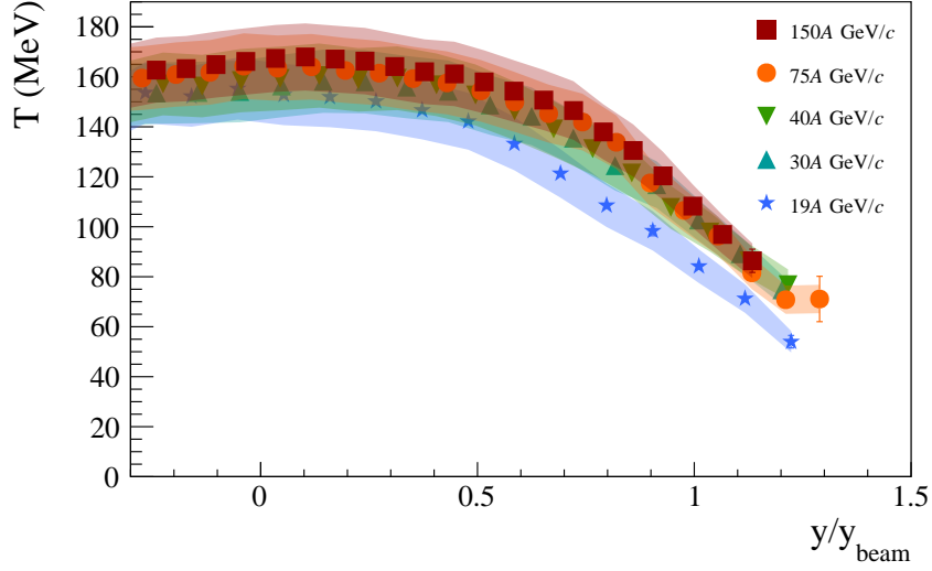
Figure 11: The inverse slope parameter T of the transverse mass spectra of negatively charged pions in central Be+Be collisions at the SPS energies as a function of rapidity divided by the beam rapidity. The fit range is 0.2 < m_T - m_\pi < 0.7 GeV. Statistical uncertainties are mostly smaller than marker size, systematic uncertainties are indicated by shaded bands.
