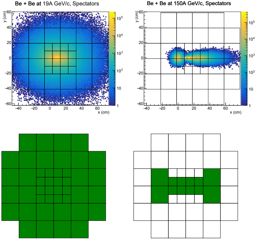
Figure 5: Upper row : Simulated impact points of particles on the front face of the PSD for beam momentum of 19A GeV/c ( left ) and 150A GeV/c ( right ). Lower row : PSD modules included in the calculation of the projectile spectator energy E_{PSD} used for event selection for beam momenta of 19A, and 30A GeV/c ( left ) and for 40A, 75A and 150A GeV/c ( right )
