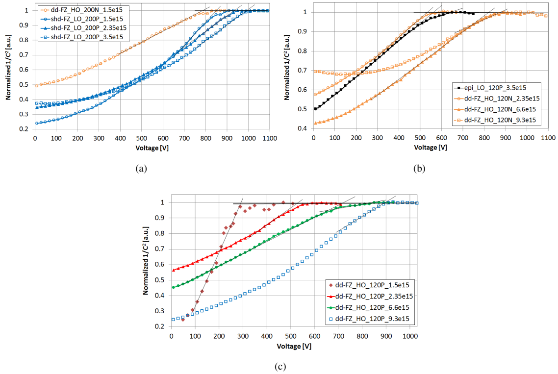
Figure 15: Measured reciprocal capacitances as a function of voltage and extracted V_{fd} -values (crossing point of two linear fits) for (a) 200N/P sensors, (b) epitaxial 120P and 120N sensors, and (c) 120P sensors corresponding to Figures 13b and 13c, respectively. Sensor identification and effective fluences (in units of n_{eq}cm^{-2} ) are indicated in the legends.
