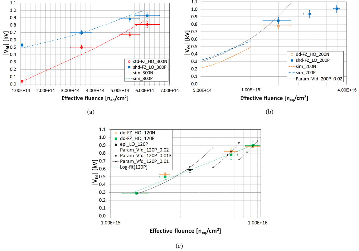
Figure 13: Evolution of full depletion voltage as a function of \Phi_{eff} for the fluence ranges anticipated for the three sensor thicknesses at HGICAL. Simulations are applied up to the neutron defect model's validated fluence limit [7]. The corresponding CV -curves are presented in Figures 14 and 15. (a) Measured (markers) and simulated (dashed curves) V_{fd}(\Phi_{eff}) for 300- \mu m thick sensors. Initial V_{fd} before irradiation for 300N and 300P were 200 V and 300 V, respectively. (b) Measured and simulated V_{fd}(\Phi_{eff}) for 200- \mu m thick sensors. V_{fd} before irradiation for 200N and 200P were 95 V and 130 V, respectively. Parametrized V_{fd}(\Phi_{eff}) was calculated using Eq. 5 with standard value of g_{eff} = 0.02 \text{ cm}^{-1} [17]. (c) Measured V_{fd}(\Phi_{eff}) for 120- \mu m thick sensors. V_{fd} before irradiation for both 120N and 120P was 50 V, while for epitaxial 120P it was 20 V. Parametrized V_{fd}(\Phi_{eff}) was calculated using Eq. 5 with standard ( 0.02 \text{ cm}^{-1} ), intermediate ( 0.013 \text{ cm}^{-1} ) and saturated ( 0.01 \text{ cm}^{-1} [17]) values of g_{eff} . The logarithmic fit value for 120P sensors is (0.33 \pm 0.11) \ln(x) - (11 \pm 4) .
