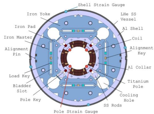
Fig. 1. The MQXF cross-section.
