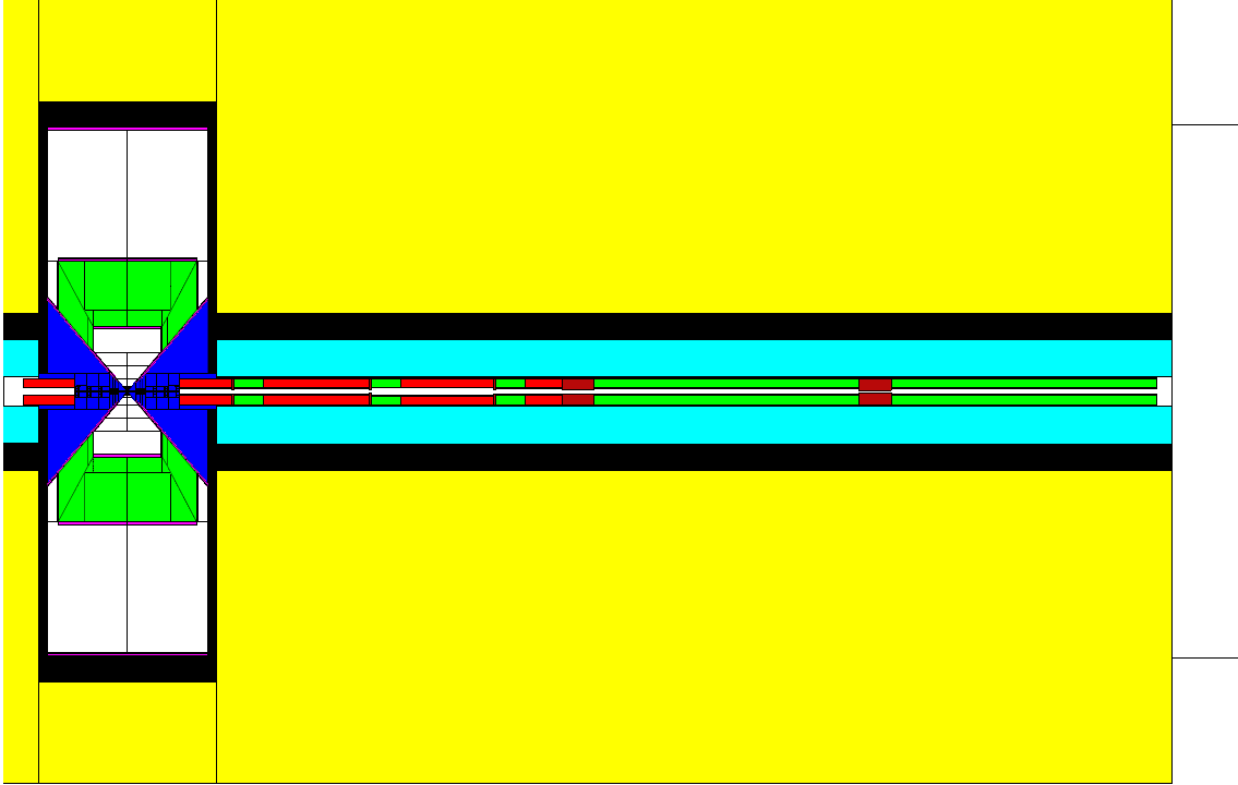
FIG. 62. Region up to 130 m from the IP, of the 2 + 2 TeV interaction region modeled in GEANT. The triangular blue regions represent tungsten shielding. On the right hand of the figure, the red areas represent quadrupoles in the beam line. The areas around the IP represent the various detector volumes used in the calculations of particle fluences. The detector (white and green areas) is 10 m in diameter and 20 m long.
