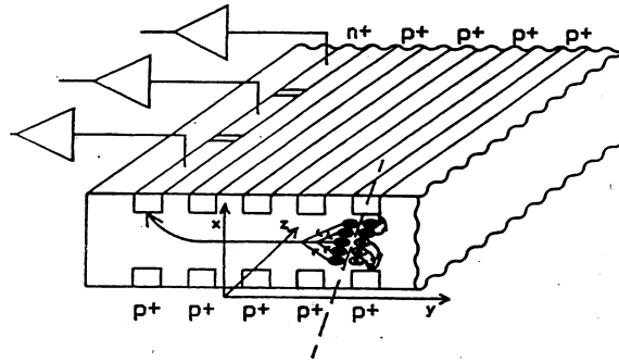
FIG. 70. Silicon drift vertex detector.
