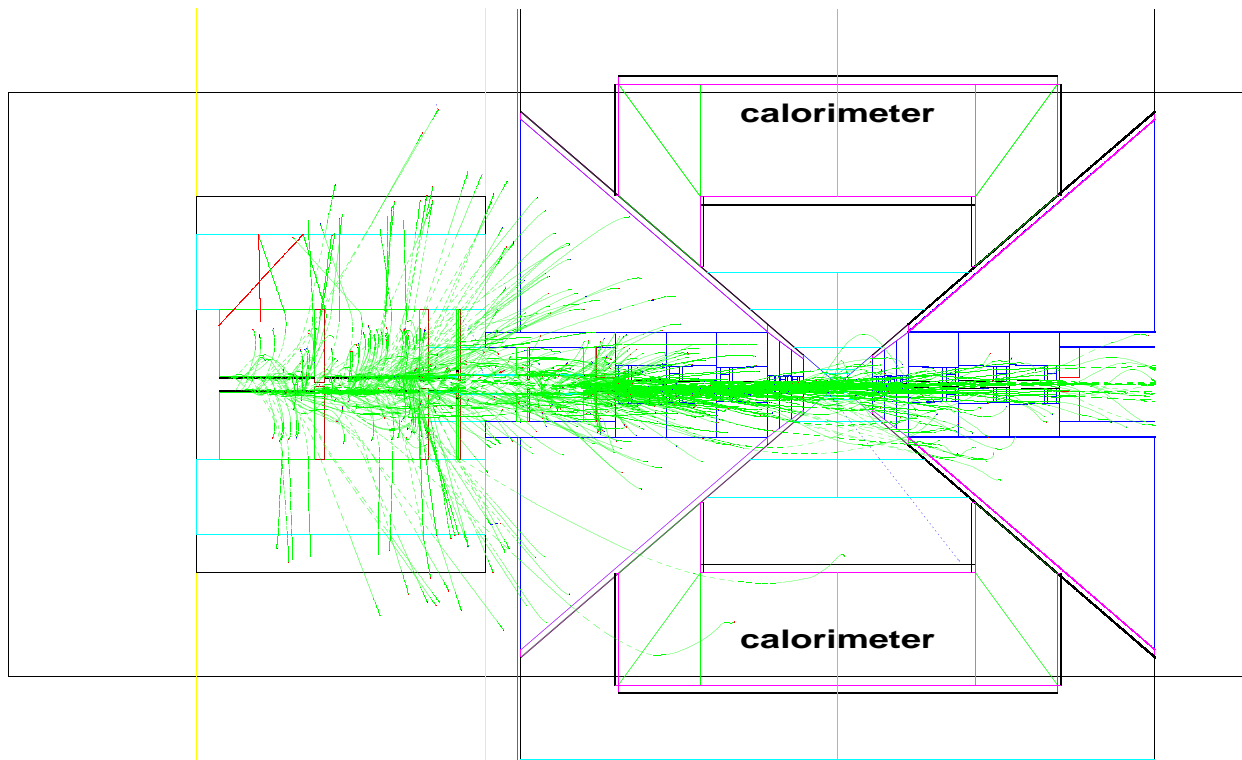
FIG. 67. Trajectories of typical Bethe-Heitler muons from their source in the shielding around the beam pipe to the detector for a 100 GeV CoM collider. As indicated in the text the scale is extremely distorted, the total horizontal length is \approx 20 m and the outer edge of the calorimeter is \approx 4 m. Notice that < 0.5\% of the tracks end in the calorimeter (see table XVII).
