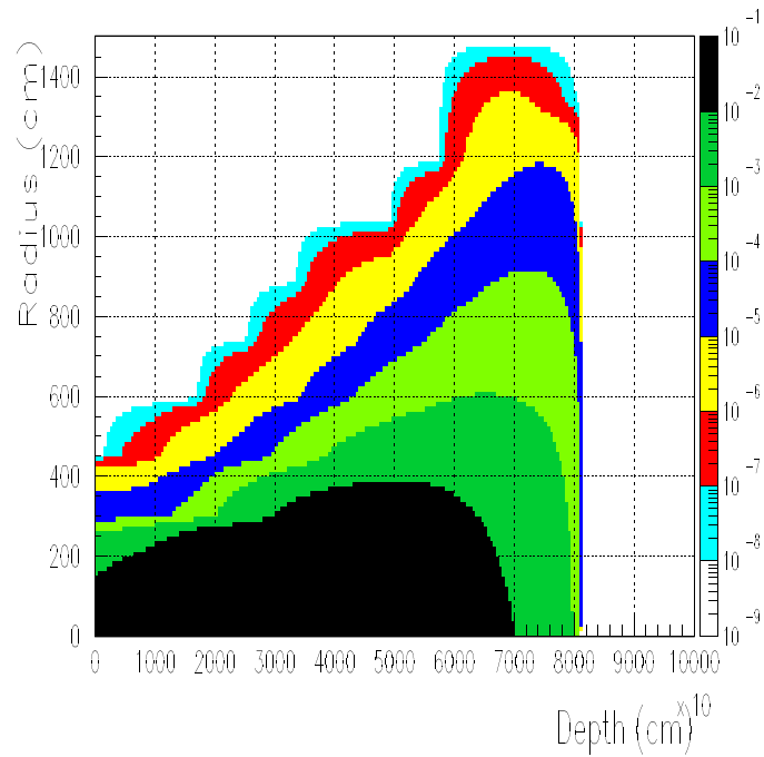
FIG. 60. Isodose contours in the soil/rock ( \rho=2.24\text{ g/cm}^3 ) for 250 GeV muons extracted at 3 \times 10^{13} per second. Right scale is dose rate in rem/s.
