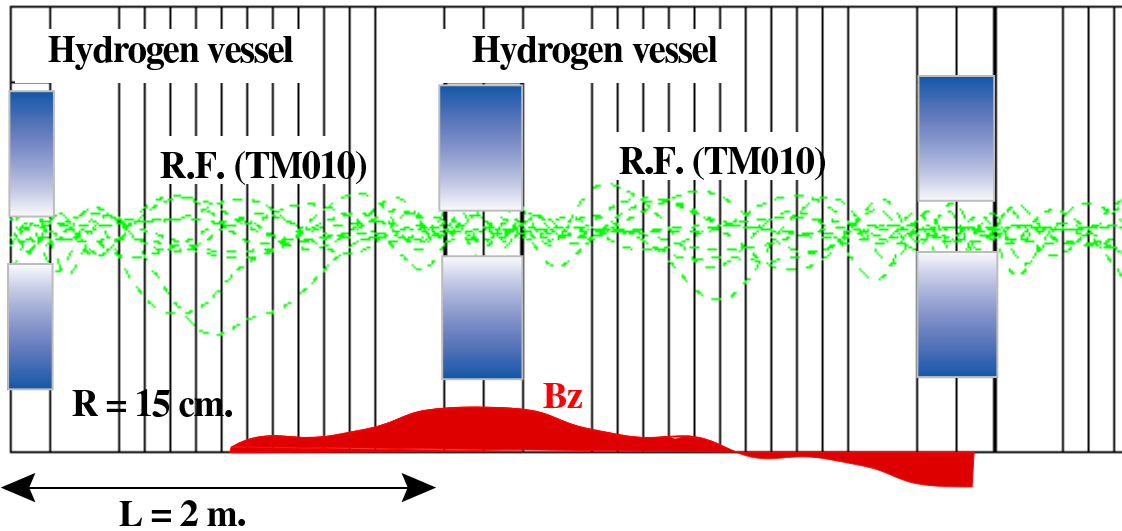
FIG. 24. GEANT simulation of muons traversing a section of the alternating solenoid cooling channel. The variation of the magnetic field B_z is shown for 1\frac{1}{2} cells of the figure.
