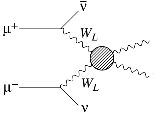
FIG. 12. Symbolic diagram for strong WW scattering.
