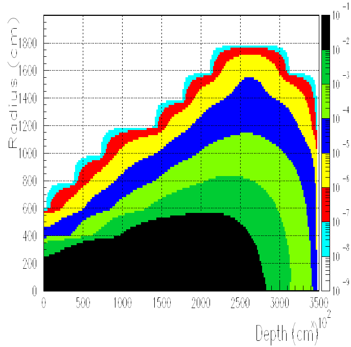
FIG. 59. Isodose contours in the soil/rock ( \rho=2.24\text{ g/cm}^3 ) for 2 TeV muons extracted at 3 \times 10^{13} per second. Right scale is dose rate in rem/s.
