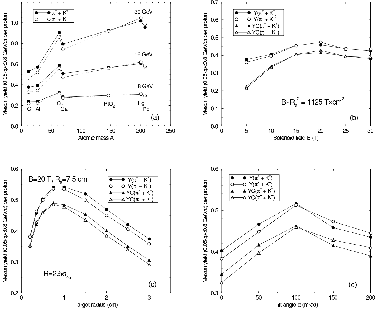
FIG. 16. Meson yield ( \pi+K ) from different targets tilted by angle \alpha in a solenoidal field B of aperture R_a as calculated with the MARS13(98) code. The target is aligned along the beam. The curves labeled YC show mesons that are transported into the decay channel. (a) Yield from a 1.5 \lambda_I , 1 cm radius target irradiated with 8, 16 and 30 GeV proton beams ( \sigma_x = \sigma_y = 4 mm) as a function of target atomic mass ( B = 20 T, R_a = 7.5 cm, \alpha = 0 ); (b) Yield from a 3 - \lambda_I , 1 cm radius gallium target tilted at \alpha = 150 mrad in a 16 GeV proton beam ( \sigma_x = \sigma_y = 4 mm) vs. solenoid field for a fixed adiabatic invariant BR_a^2 ; (c) Yield as a function of radius of a 3 \lambda_I gallium target in a 16 GeV proton beam ( \sigma_x = \sigma_y = 4 mm, B = 20 T, R_a = 7.5 cm, \alpha = 100 mrad); (d) Yield from a 3 \lambda_I , 1 cm radius gallium target vs. tilt angle between the axis of the capture solenoid and the proton beam for a 16 GeV proton beam ( \sigma_x = \sigma_y = 4 mm, B = 20 T, R_a = 7.5 cm).
