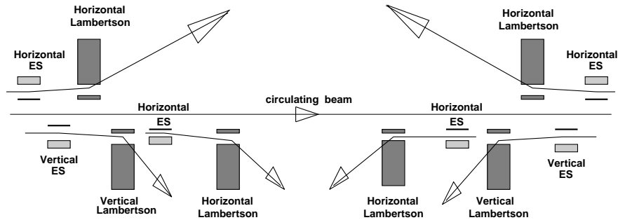
FIG. 50. Schematic view of a \mu^+\mu^- collider beam halo extraction.
