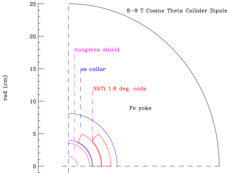
FIG. 53. Cross Section of a baseline dipole magnet suitable for the 100 GeV collider.
